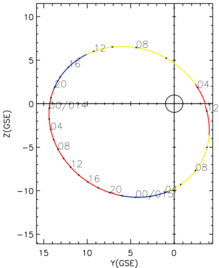
CLUSTER 2 orbit 2006 013 (01/13) 03:11 UT to 2006 015 (01/15) 12:16 UT
