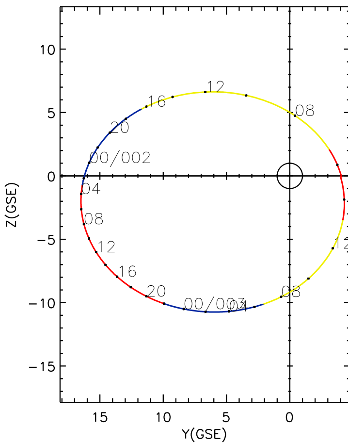
CLUSTER 2 orbit 2006 001 (01/01) 05:36 UT to 2006 003 (01/03) 14:46 UT
