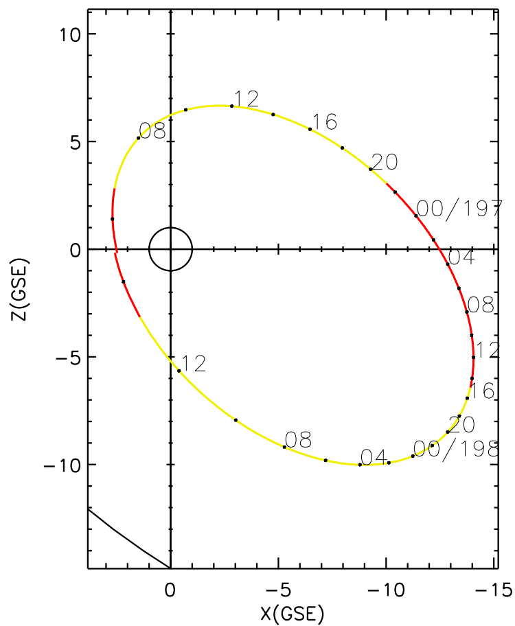
CLUSTER 2 orbit 2005 196 (07/15) 05:25 UT to 2005 198 (07/17) 14:30 UT
