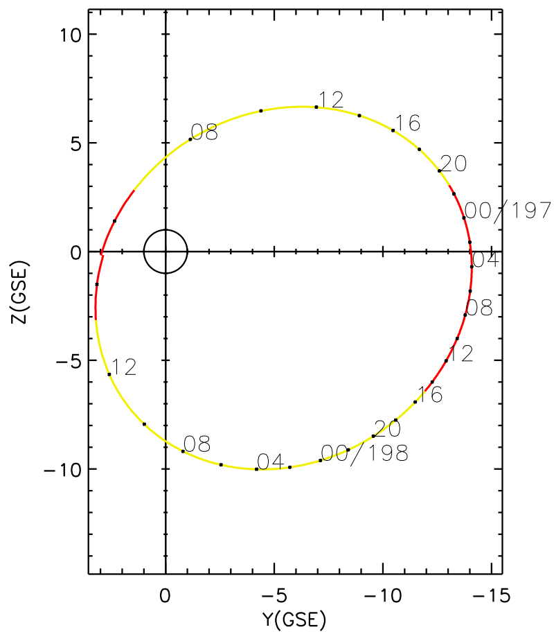
CLUSTER 2 orbit 2005 196 (07/15) 05:25 UT to 2005 198 (07/17) 14:30 UT
