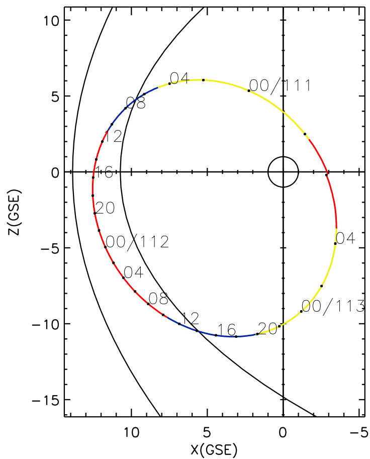
CLUSTER 2 orbit 2005 110 (04/20) 20:56 UT to 2005 113 (04/23) 06:01 UT
