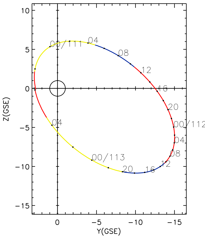
CLUSTER 2 orbit 2005 110 (04/20) 20:56 UT to 2005 113 (04/23) 06:01 UT
