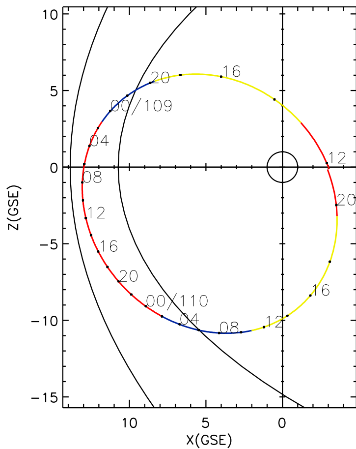
CLUSTER 2 orbit 2005 108 (04/18) 11:51 UT to 2005 110 (04/20) 20:56 UT
