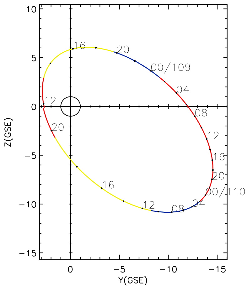
CLUSTER 2 orbit 2005 108 (04/18) 11:51 UT to 2005 110 (04/20) 20:56 UT
