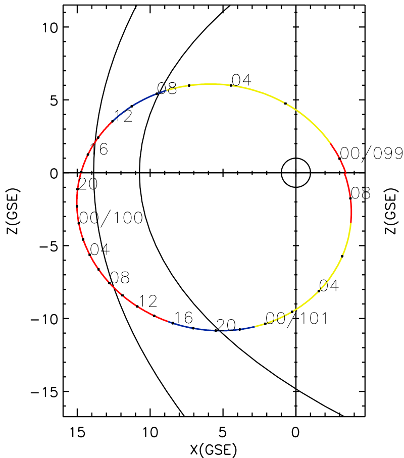
CLUSTER 2 orbit 2005 098 (04/08) 23:36 UT to 2005 101 (04/11) 08:41 UT
