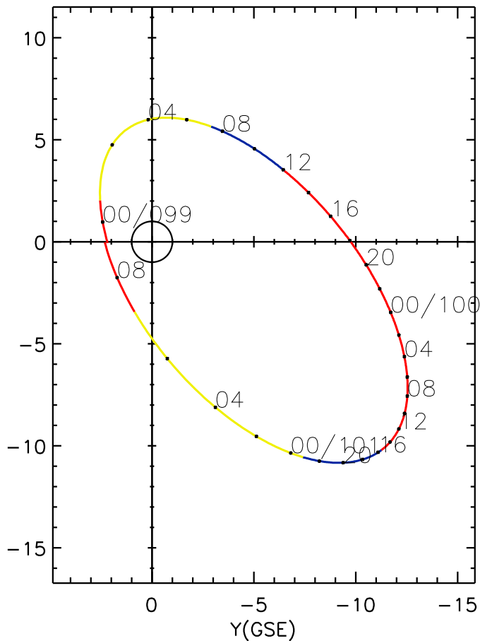
CLUSTER 2 orbit 2005 098 (04/08) 23:36 UT to 2005 101 (04/11) 08:41 UT
