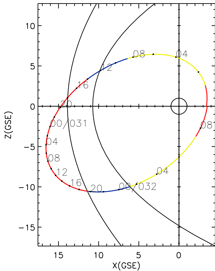
CLUSTER 2 orbit 2005 030 (01/30) 00:01 UT to 2005 032 (02/01) 09:06 UT
