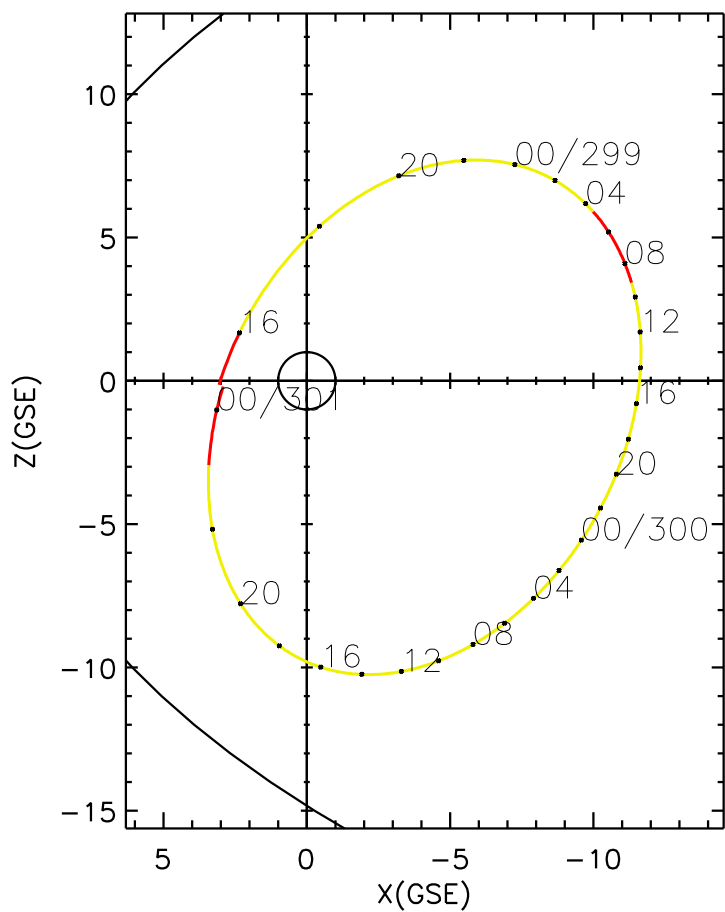
CLUSTER 2 orbit 2004 298 (10/24) 15:15 UT to 2004 301 (10/27) 00:20 UT
