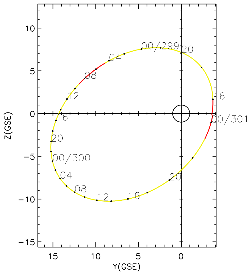
CLUSTER 2 orbit 2004 298 (10/24) 15:15 UT to 2004 301 (10/27) 00:20 UT
