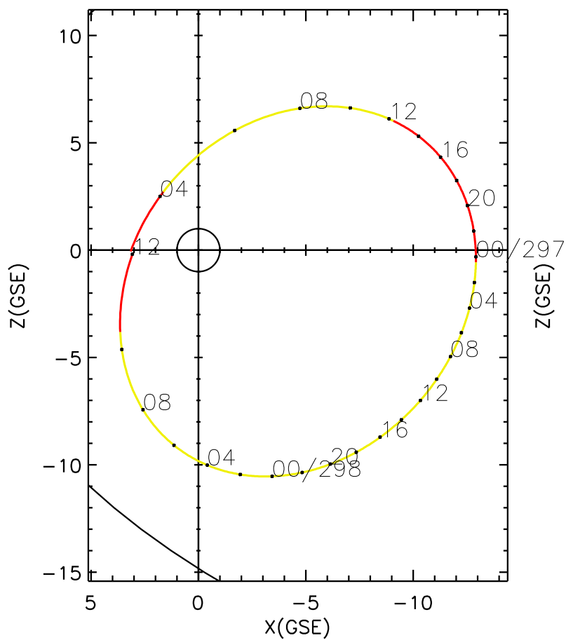
CLUSTER 2 orbit 2004 296 (10/22) 02:56 UT to 2004 298 (10/24) 12:01 UT
