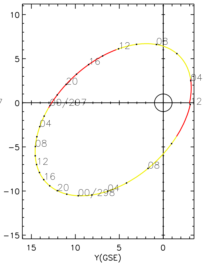
CLUSTER 2 orbit 2004 296 (10/22) 02:56 UT to 2004 298 (10/24) 12:01 UT
