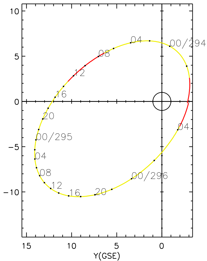
CLUSTER 2 orbit 2004 293 (10/19) 20:10 UT to 2004 296 (10/22) 05:15 UT
