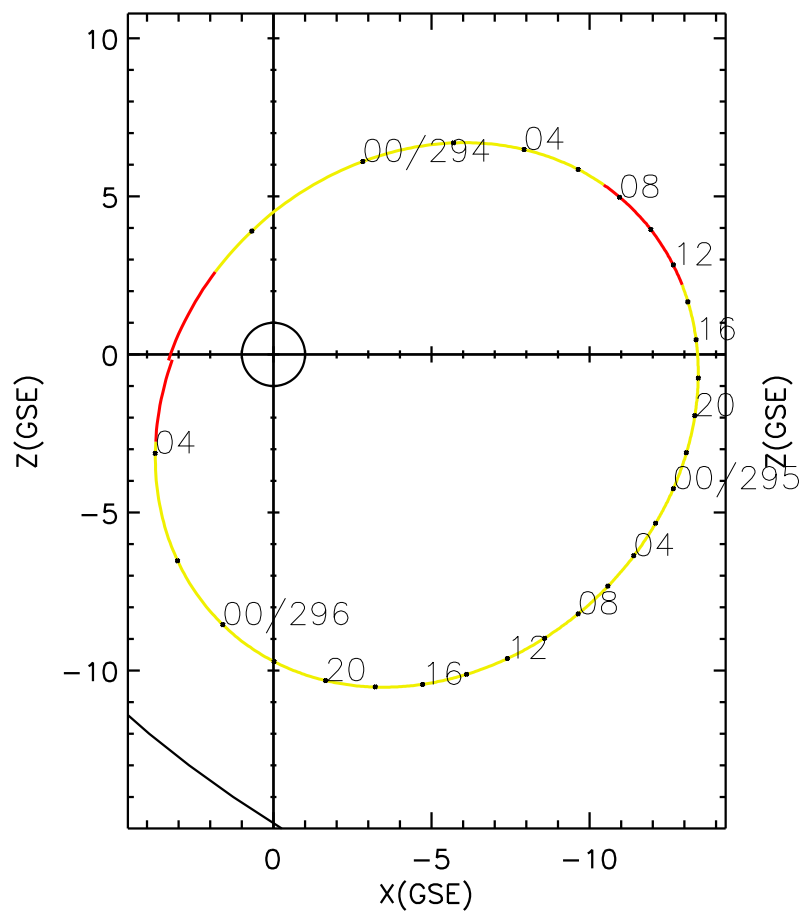
CLUSTER 2 orbit 2004 293 (10/19) 20:10 UT to 2004 296 (10/22) 05:15 UT
