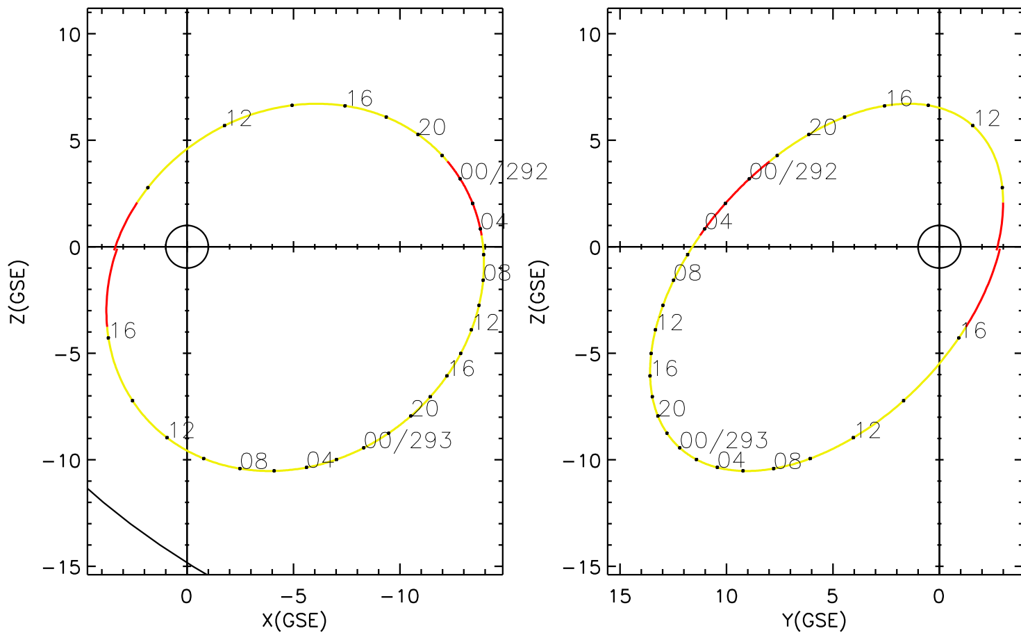
CLUSTER 2 orbit 2004 291 (10/17) 08:46 UT to 2004 293 (10/19) 17:51 UT
