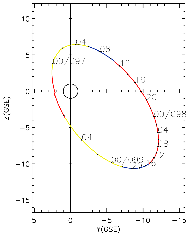
CLUSTER 2 orbit 2004 096 (04/05) 22:16 UT to 2004 099 (04/08) 07:21 UT
