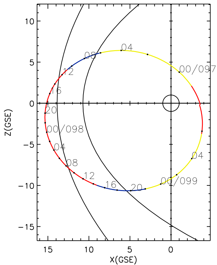
CLUSTER 2 orbit 2004 096 (04/05) 22:16 UT to 2004 099 (04/08) 07:21 UT
