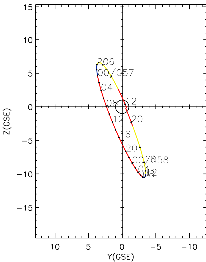
CLUSTER 2 orbit 2004 056 (02/25) 11:46 UT to 2004 058 (02/27) 20:51 UT
