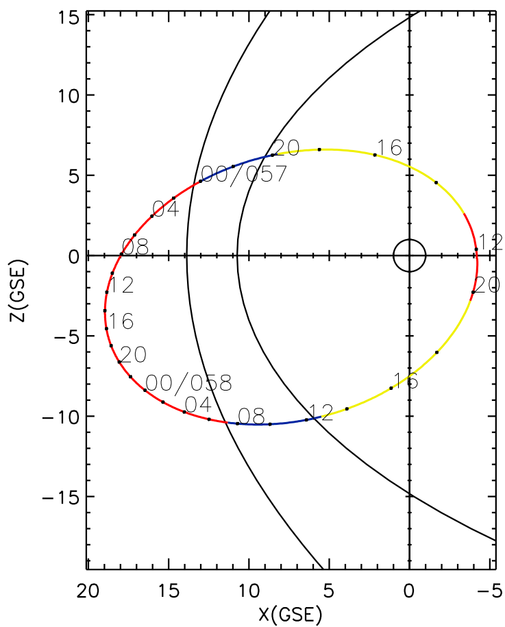
CLUSTER 2 orbit 2004 056 (02/25) 11:46 UT to 2004 058 (02/27) 20:51 UT
