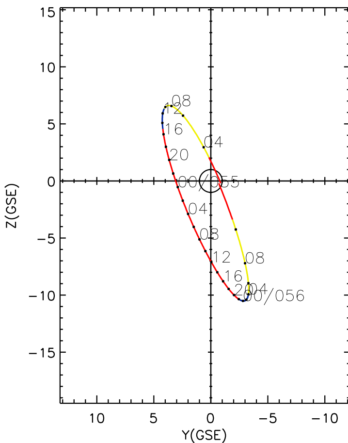
CLUSTER 2 orbit 2004 054 (02/23) 02:41 UT to 2004 056 (02/25) 11:46 UT
