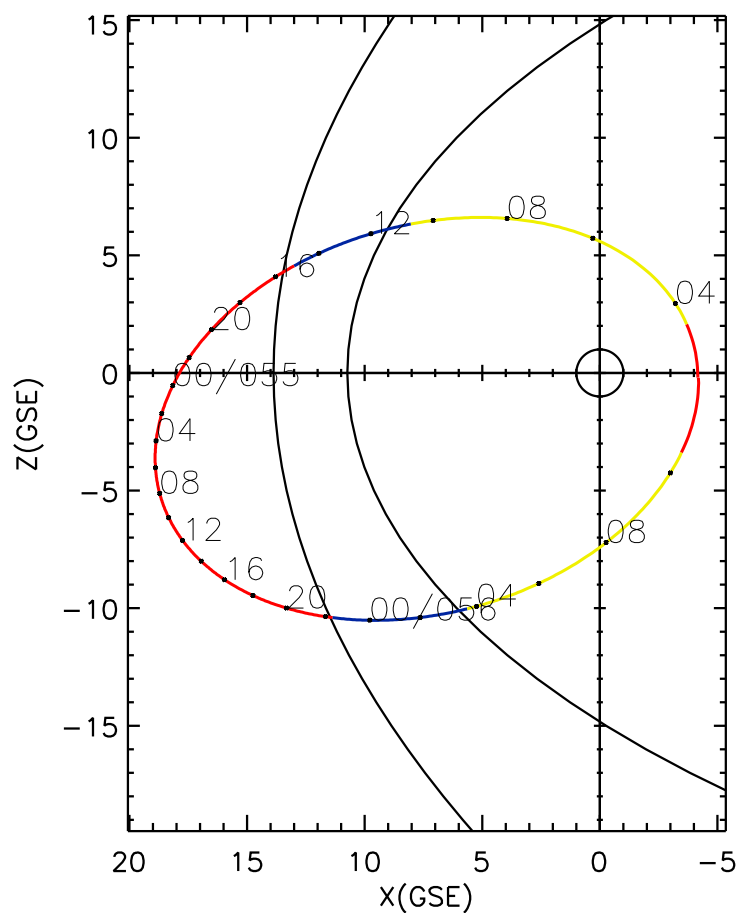
CLUSTER 2 orbit 2004 054 (02/23) 02:41 UT to 2004 056 (02/25) 11:46 UT
