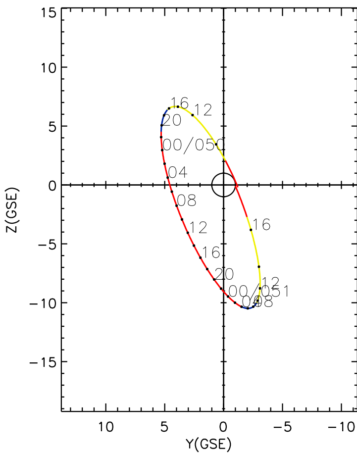
CLUSTER 2 orbit 2004 049 (02/18) 08:26 UT to 2004 051 (02/20) 17:36 UT
