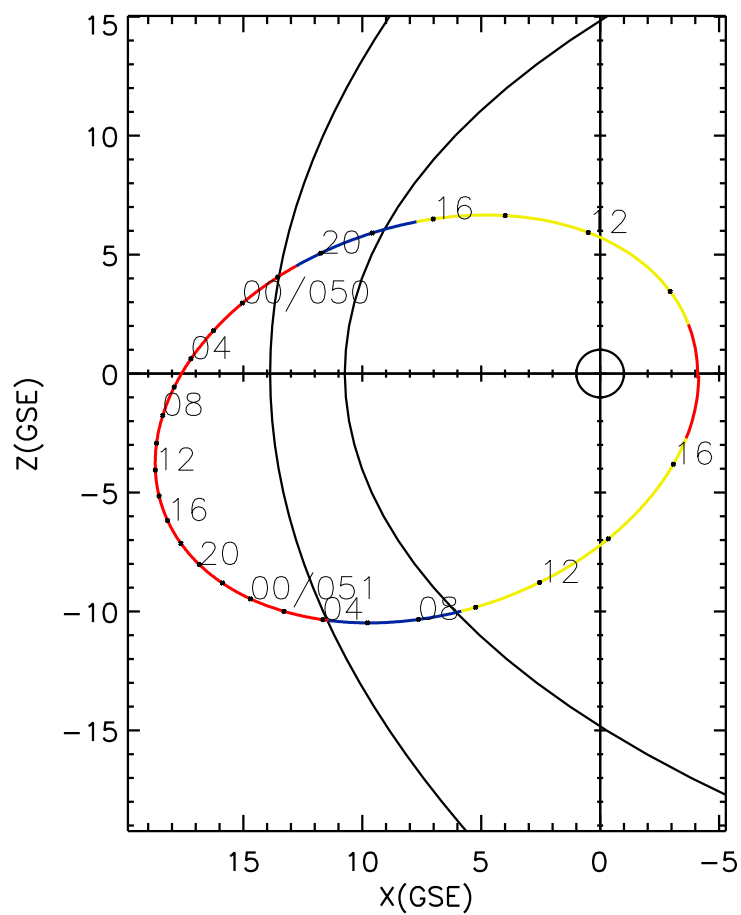
CLUSTER 2 orbit 2004 049 (02/18) 08:26 UT to 2004 051 (02/20) 17:36 UT
