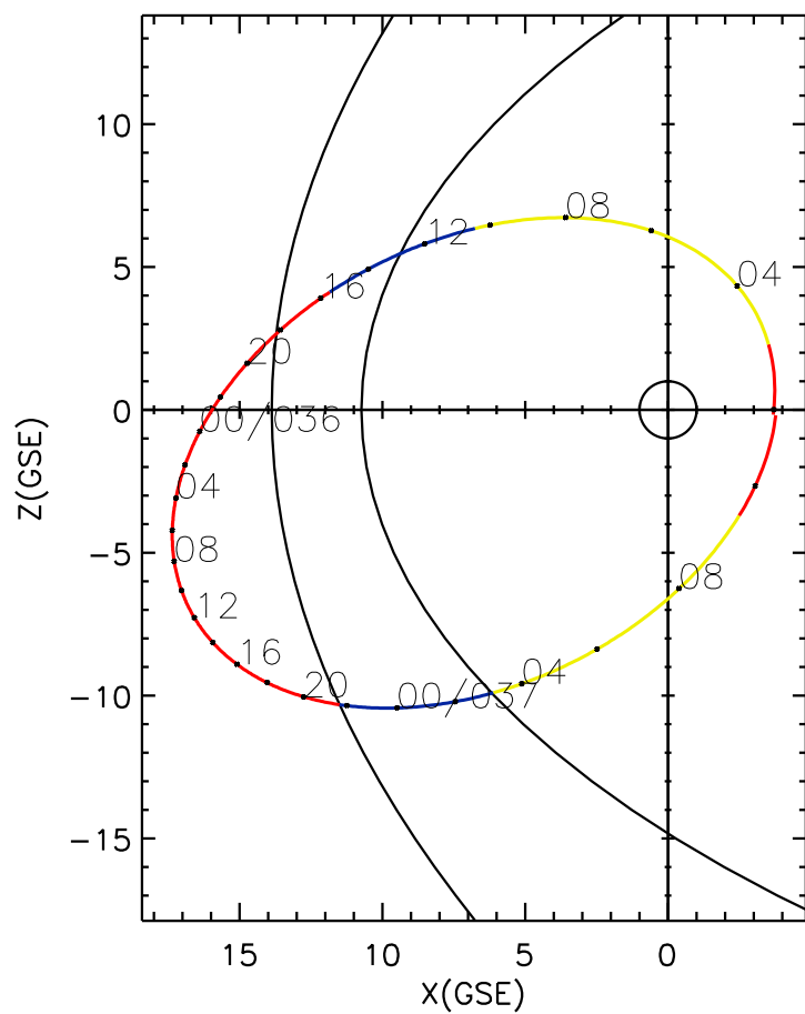
CLUSTER 2 orbit 2004 035 (02/04) 01:56 UT to 2004 037 (02/06) 11:01 UT
