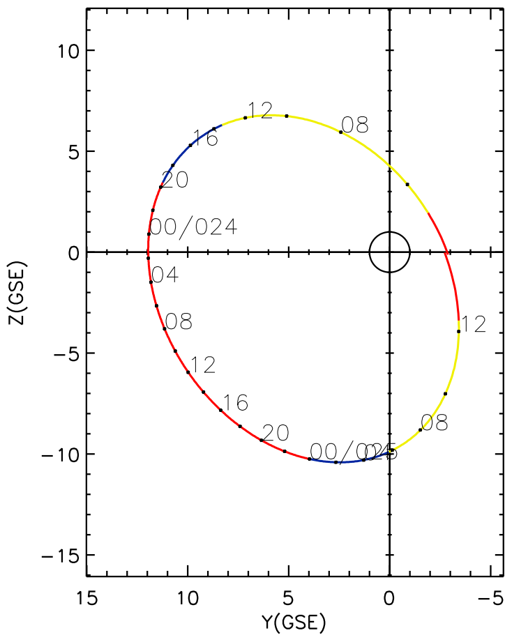
CLUSTER 2 orbit 2004 023 (01/23) 04:31 UT to 2004 025 (01/25) 13:41 UT
