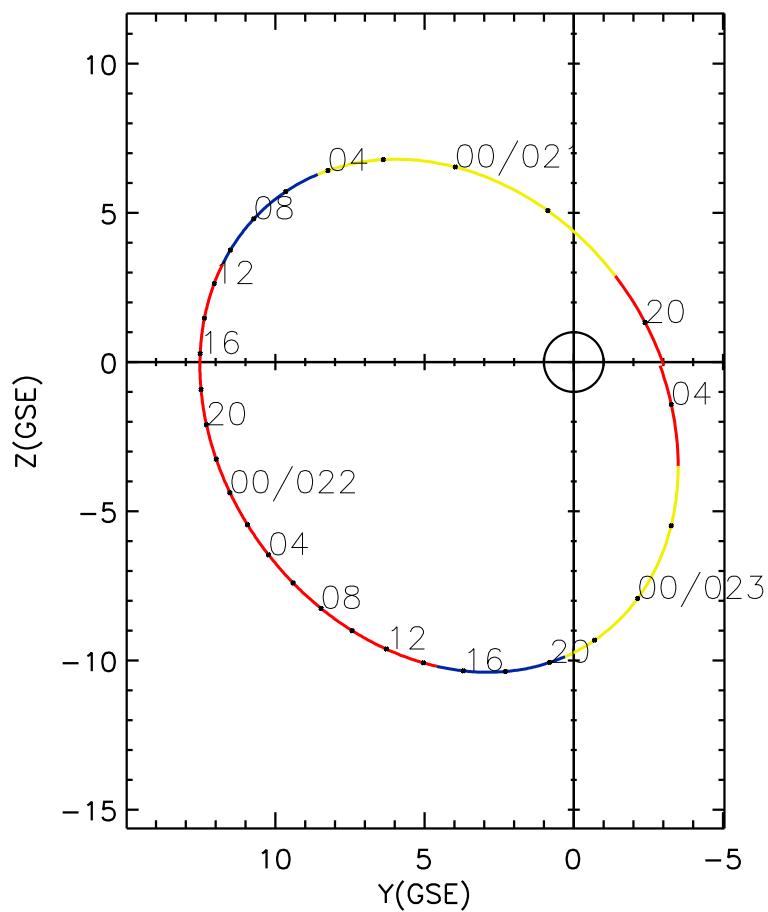
CLUSTER 2 orbit 2004 020 (01/20) 19:25 UT to 2004 023 (01/23) 04:31 UT
