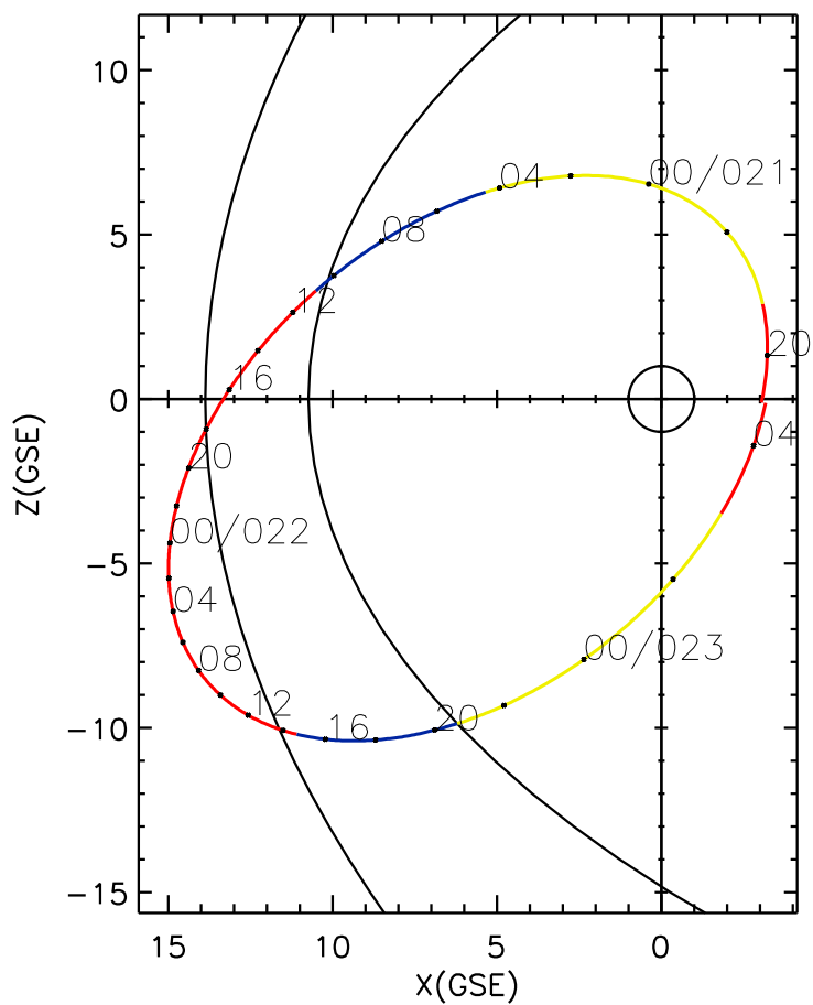
CLUSTER 2 orbit 2004 020 (01/20) 19:25 UT to 2004 023 (01/23) 04:31 UT
