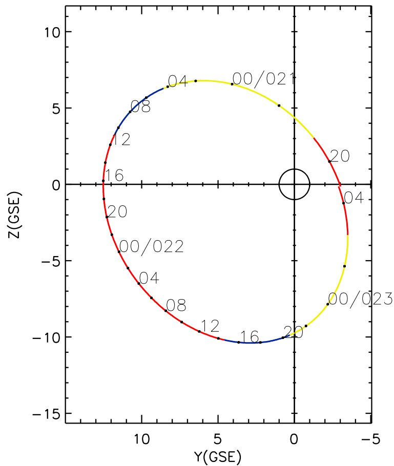
CLUSTER 2 orbit 2004 020 (01/20) 19:21 UT to 2004 023 (01/23) 04:26 UT
