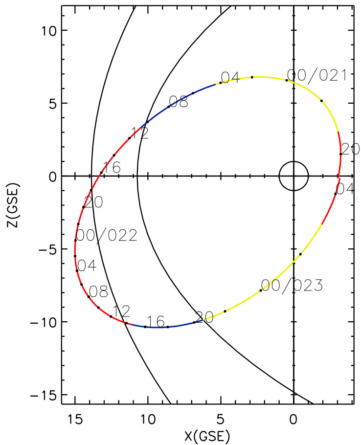
CLUSTER 2 orbit 2004 020 (01/20) 19:21 UT to 2004 023 (01/23) 04:26 UT
