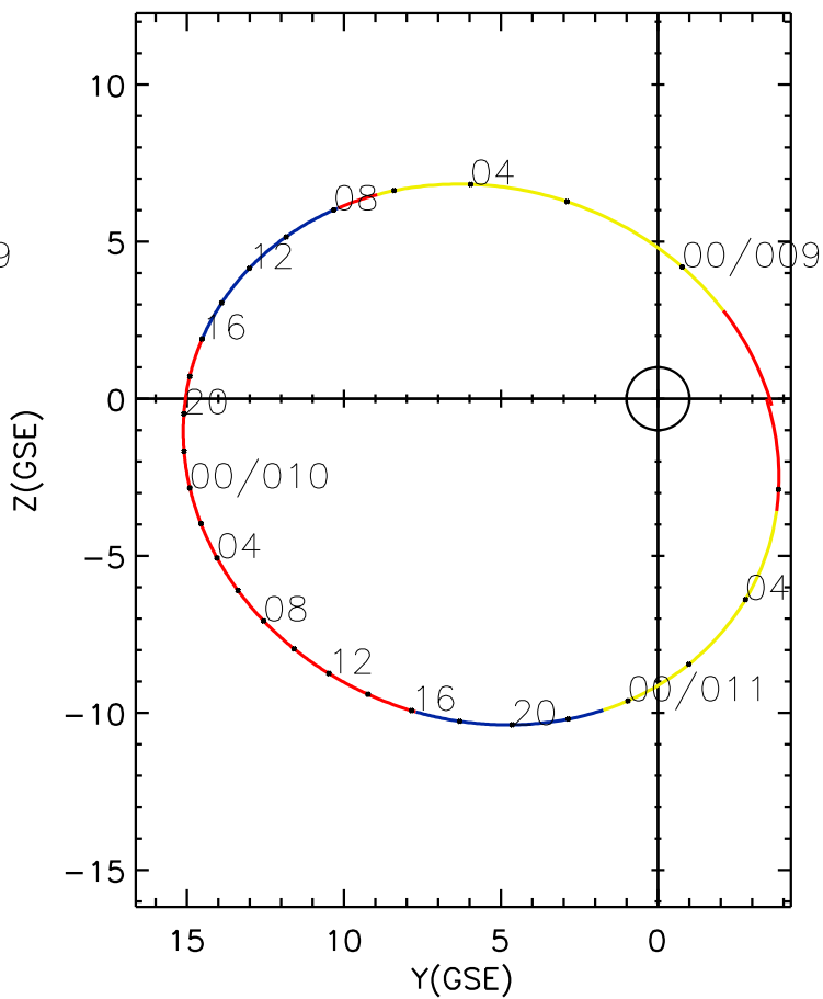
CLUSTER 2 orbit 2004 008 (01/08) 22:01 UT to 2004 011 (01/11) 07:11 UT
