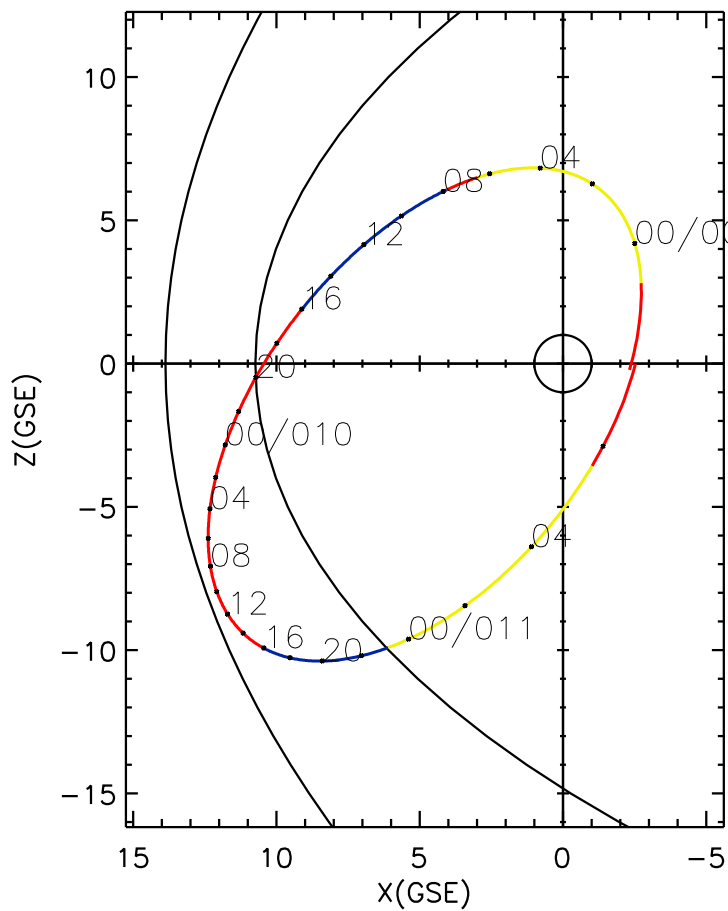
CLUSTER 2 orbit 2004 008 (01/08) 22:01 UT to 2004 011 (01/11) 07:11 UT
