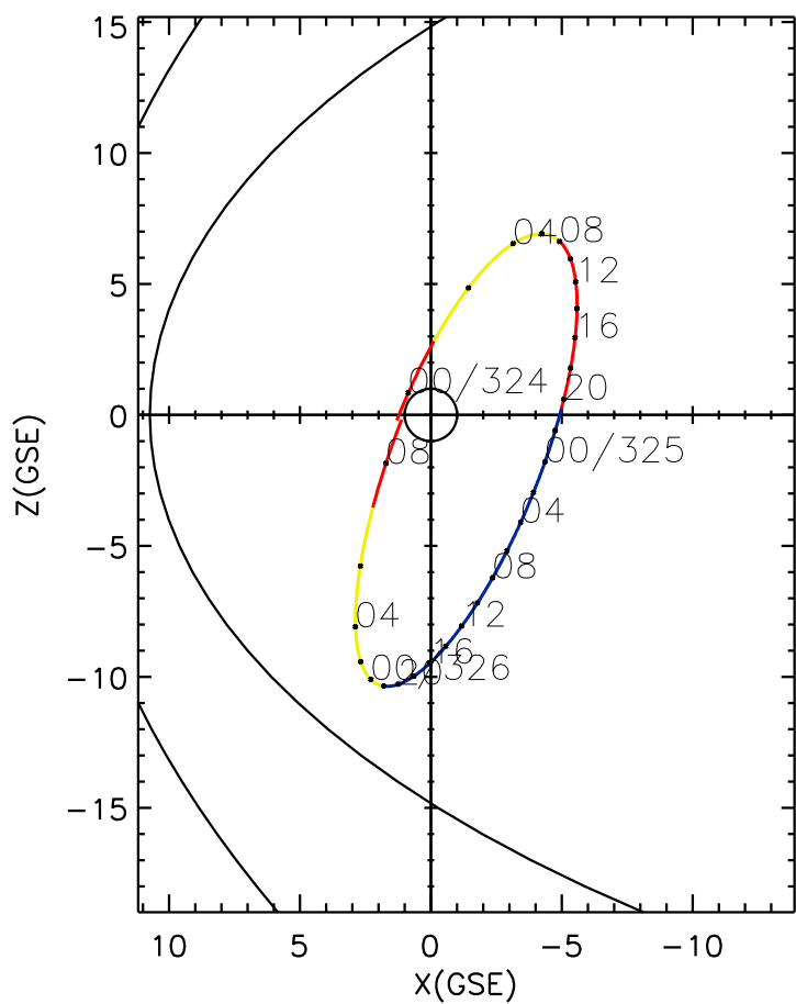
CLUSTER 2 orbit 2003 323 (11/19) 23:35 UT to 2003 326 (11/22) 08:40 UT
