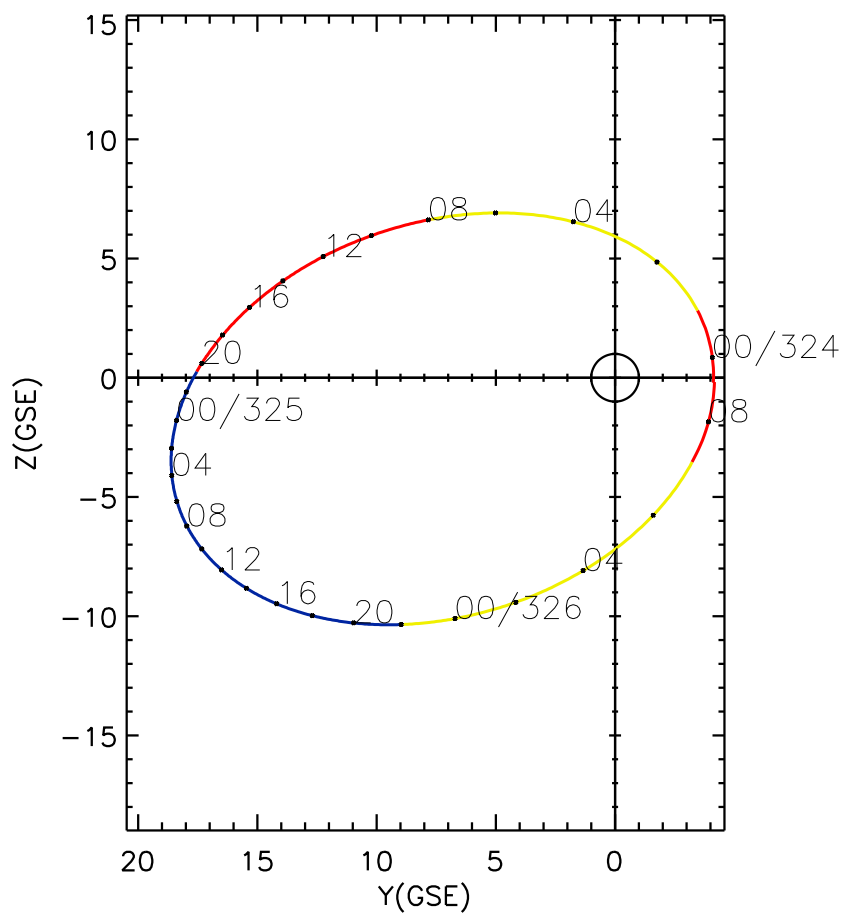
CLUSTER 2 orbit 2003 323 (11/19) 23:35 UT to 2003 326 (11/22) 08:40 UT
