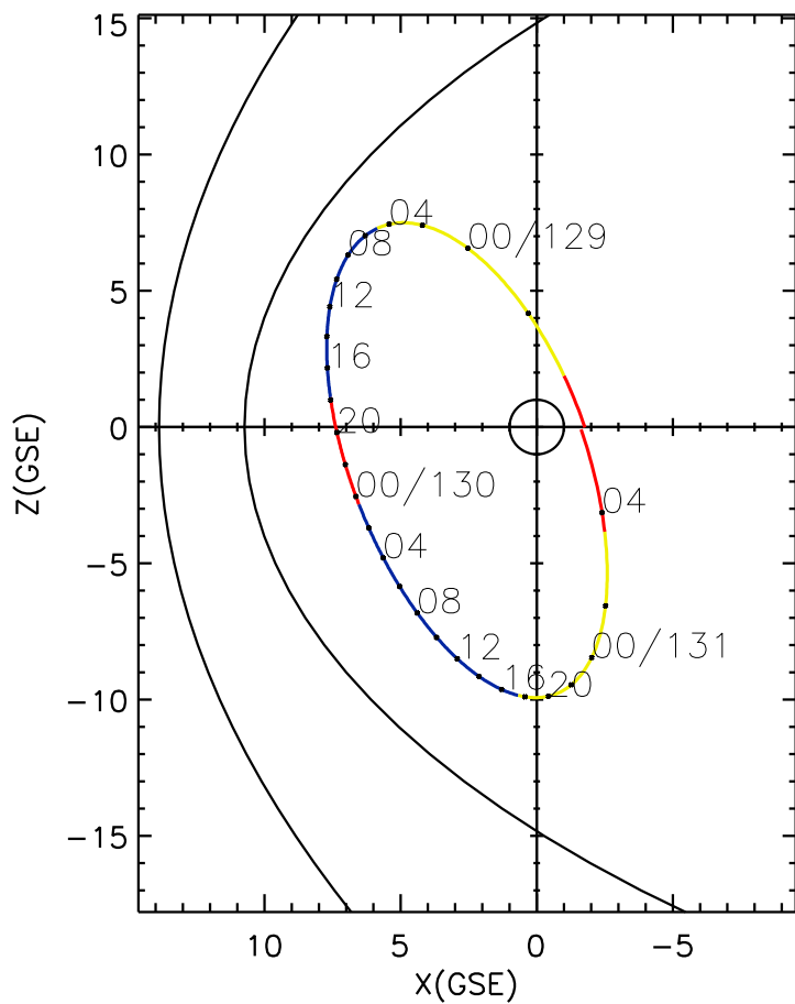
CLUSTER 2 orbit 2003 128 (05/08) 20:10 UT to 2003 131 (05/11) 05:15 UT
