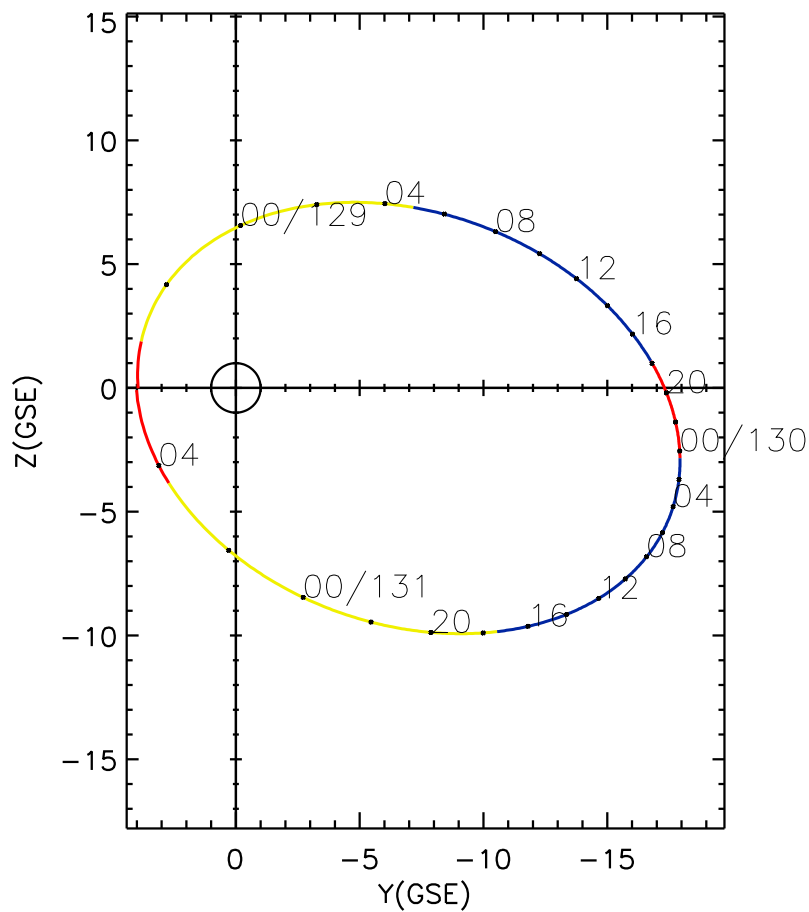
CLUSTER 2 orbit 2003 128 (05/08) 20:10 UT to 2003 131 (05/11) 05:15 UT
