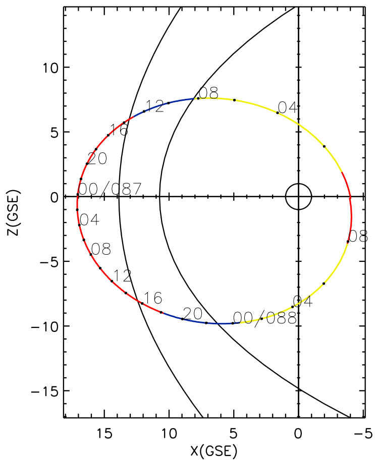
CLUSTER 2 orbit 2003 086 (03/27) 00:15 UT to 2003 088 (03/29) 09:25 UT
