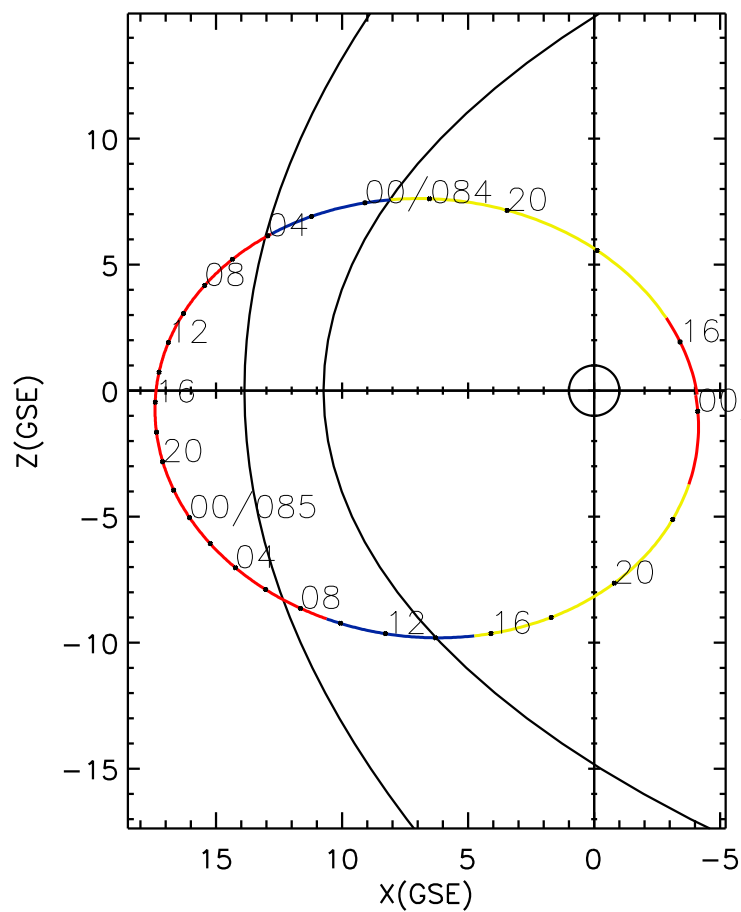
CLUSTER 2 orbit 2003 083 (03/24) 15:10 UT to 2003 086 (03/27) 00:15 UT
