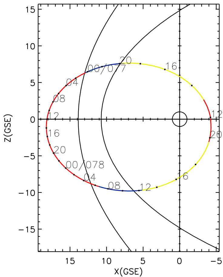
CLUSTER 2 orbit 2003 076 (03/17) 11:50 UT to 2003 078 (03/19) 21:00 UT
