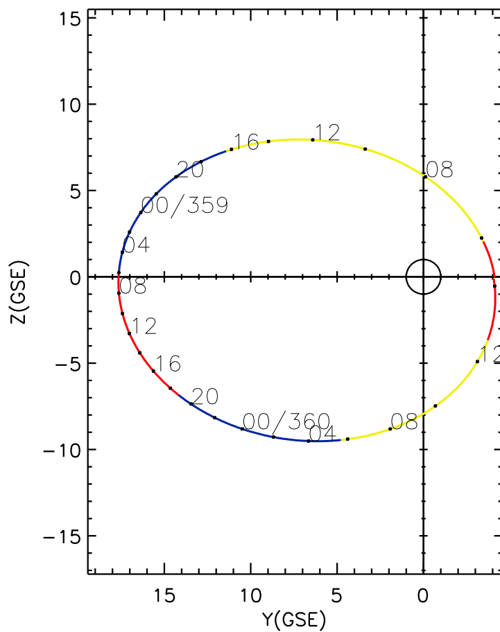
CLUSTER 2 orbit 2002 358 (12/24) 05:05 UT to 2002 360 (12/26) 14:10 UT
