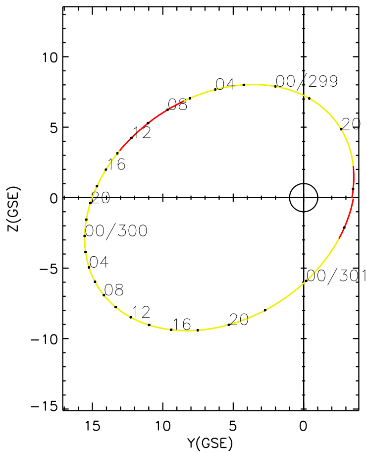
CLUSTER 2 orbit 2002 298 (10/25) 17:45 UT to 2002 301 (10/28) 02:50 UT
