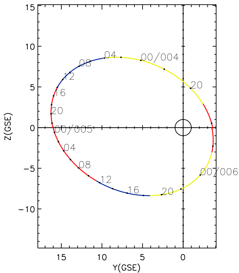
CLUSTER 2 orbit 2002 003 (01/03) 17:45 UT to 2002 006 (01/06) 02:55 UT
