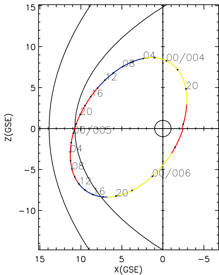
CLUSTER 2 orbit 2002 003 (01/03) 17:45 UT to 2002 006 (01/06) 02:55 UT
