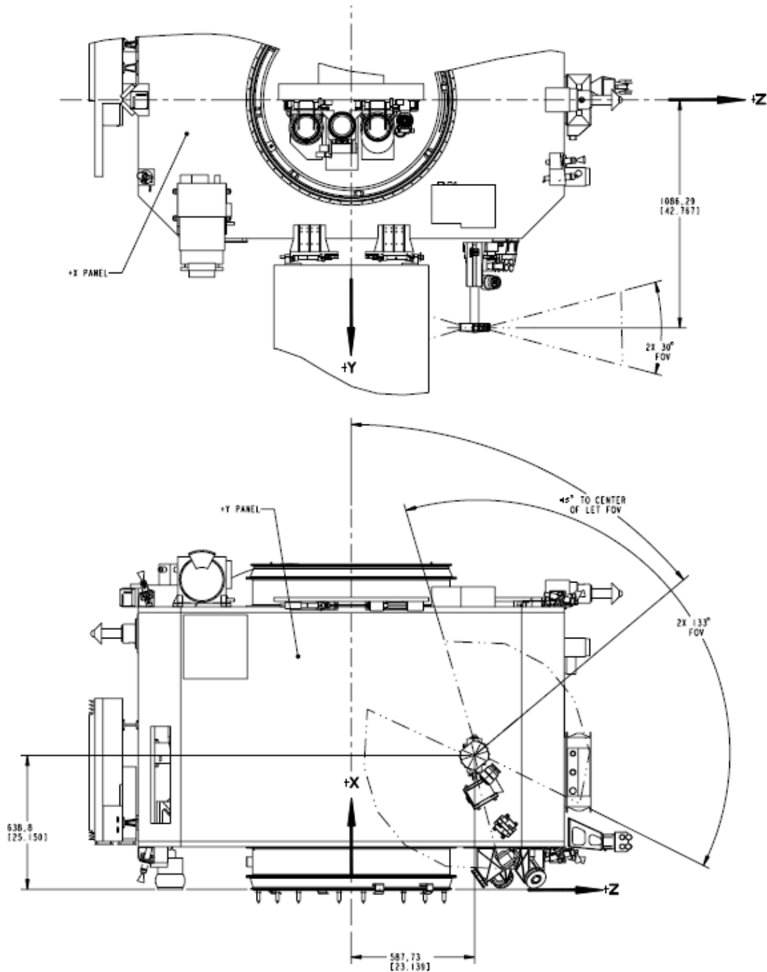
Figure A3.1: LET mounting and orientation on the Ahead Spacecraft, showing S/C X, Y, and Z axes. For illustration purposes only, positions and dimensions not exact.
