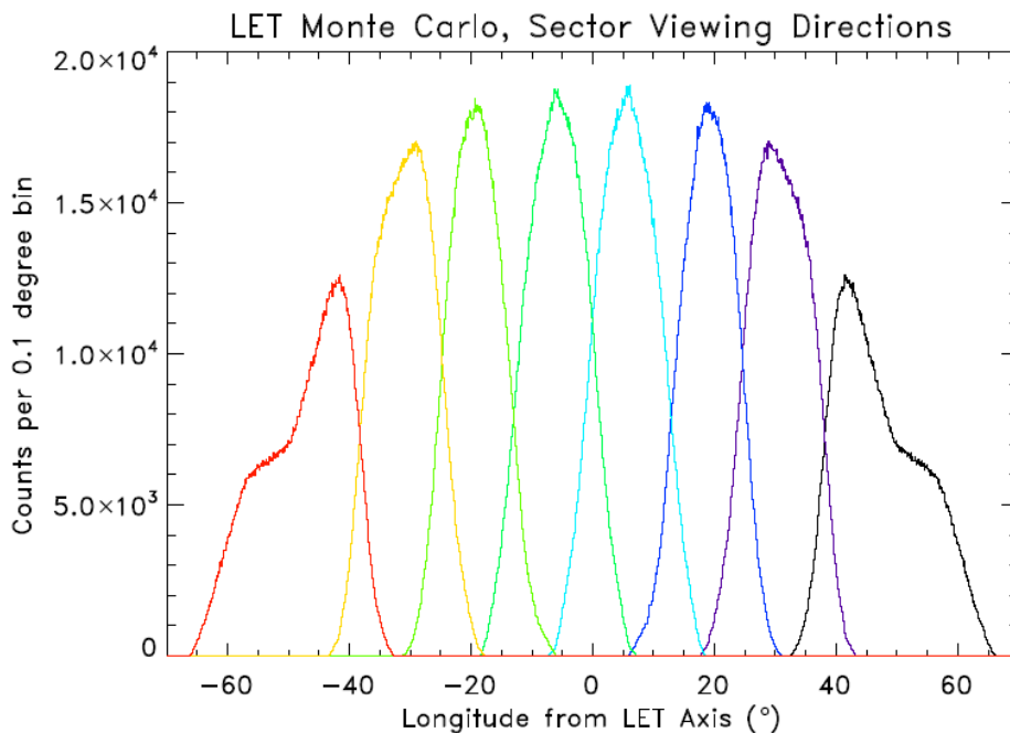
Figure A3.2: Coverage in longitudinal angle for each of the LET sectors.
