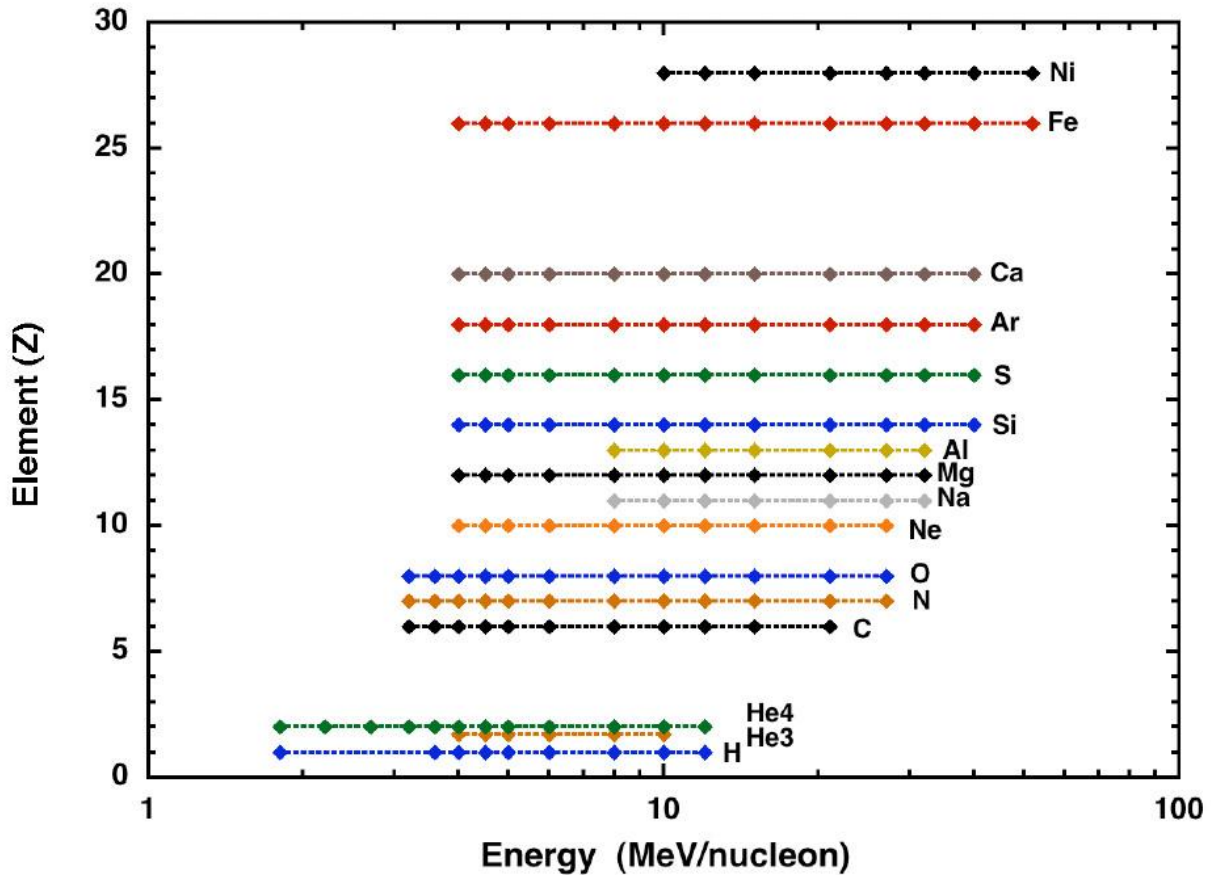
Figure 2: LET Instrument Species and Energy-range. The diamonds represent the boundaries between energy bands.
