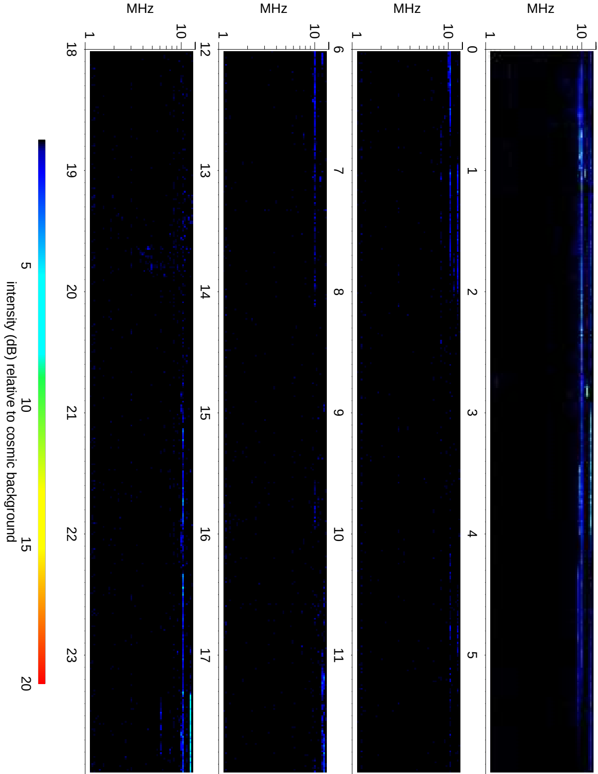
Wind Waves RAD2 receiver: 2019/10/10
