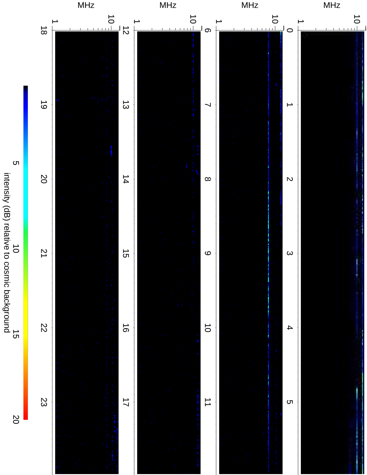
Wind Waves RAD2 receiver: 2018/11/15
