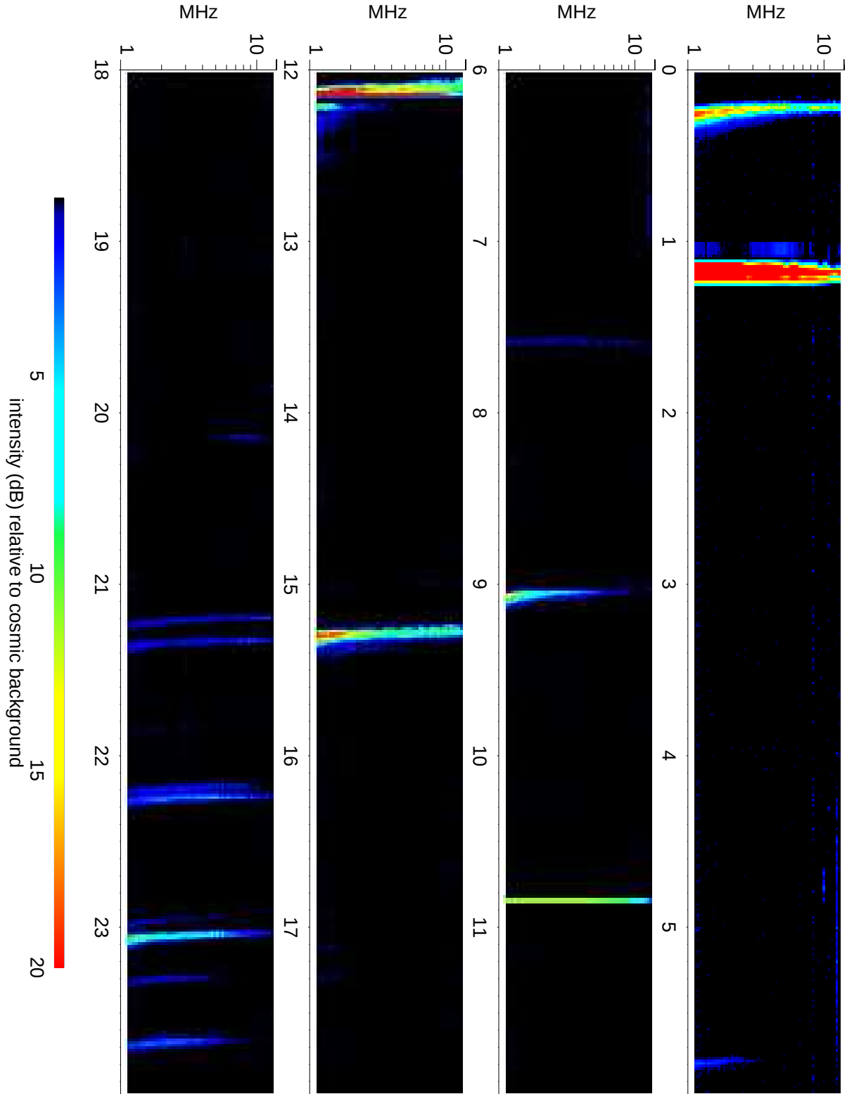
Wind Waves RAD2 receiver: 2014/08/24
