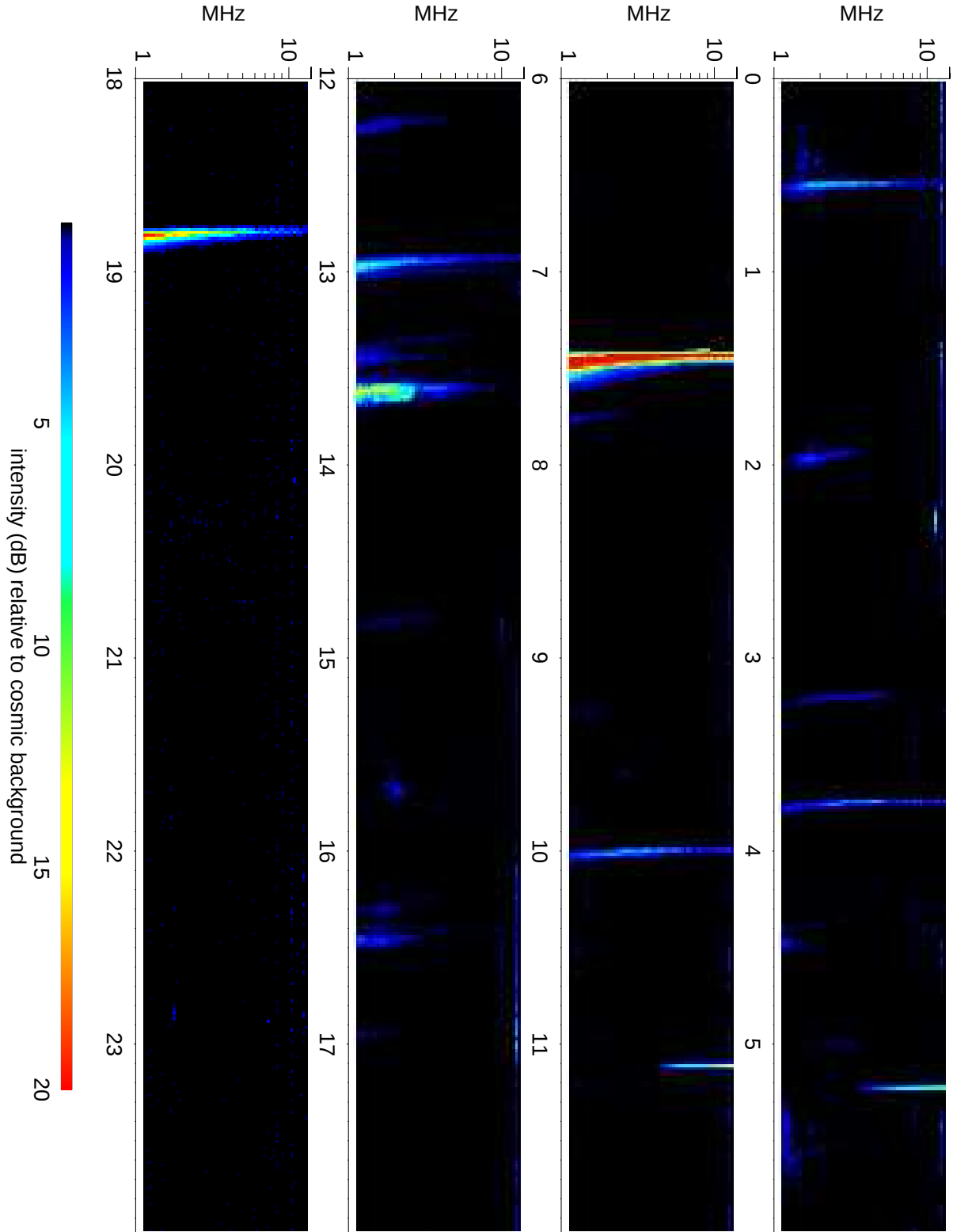
Wind Waves RAD2 receiver: 2012/12/12
