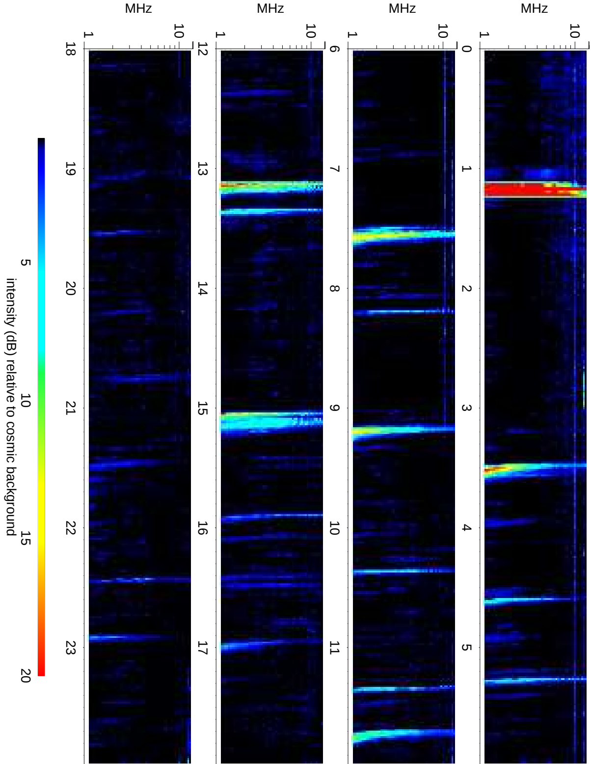
Wind Waves RAD2 receiver: 2012/07/14
