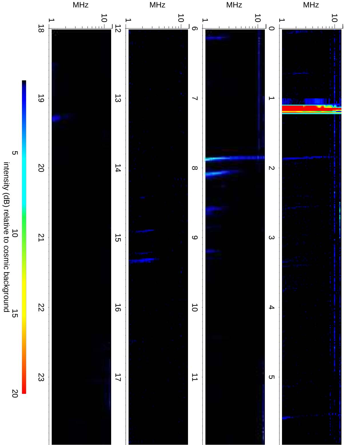
Wind Waves RAD2 receiver: 2012/06/10
