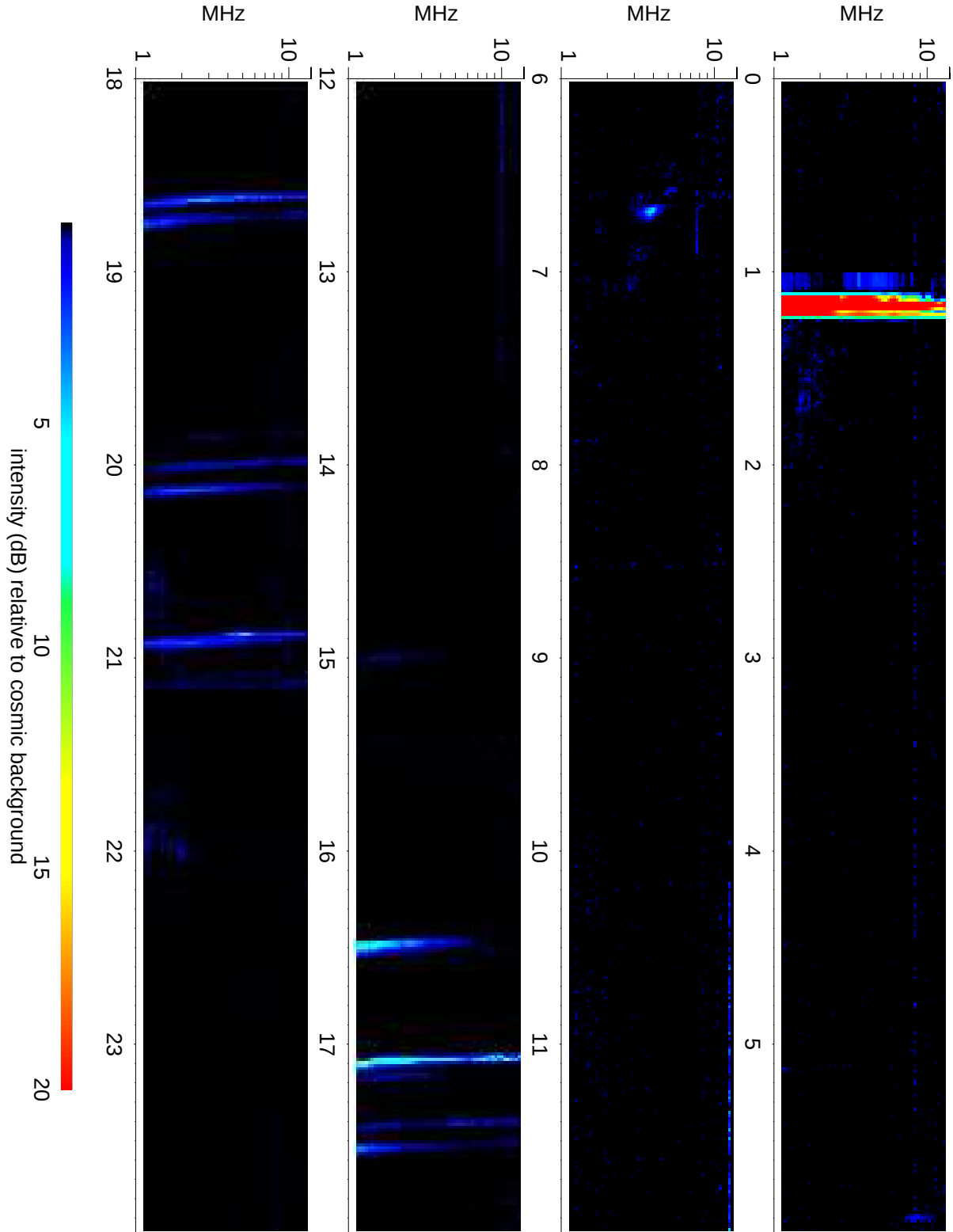
Wind Waves RAD2 receiver: 2012/01/26
