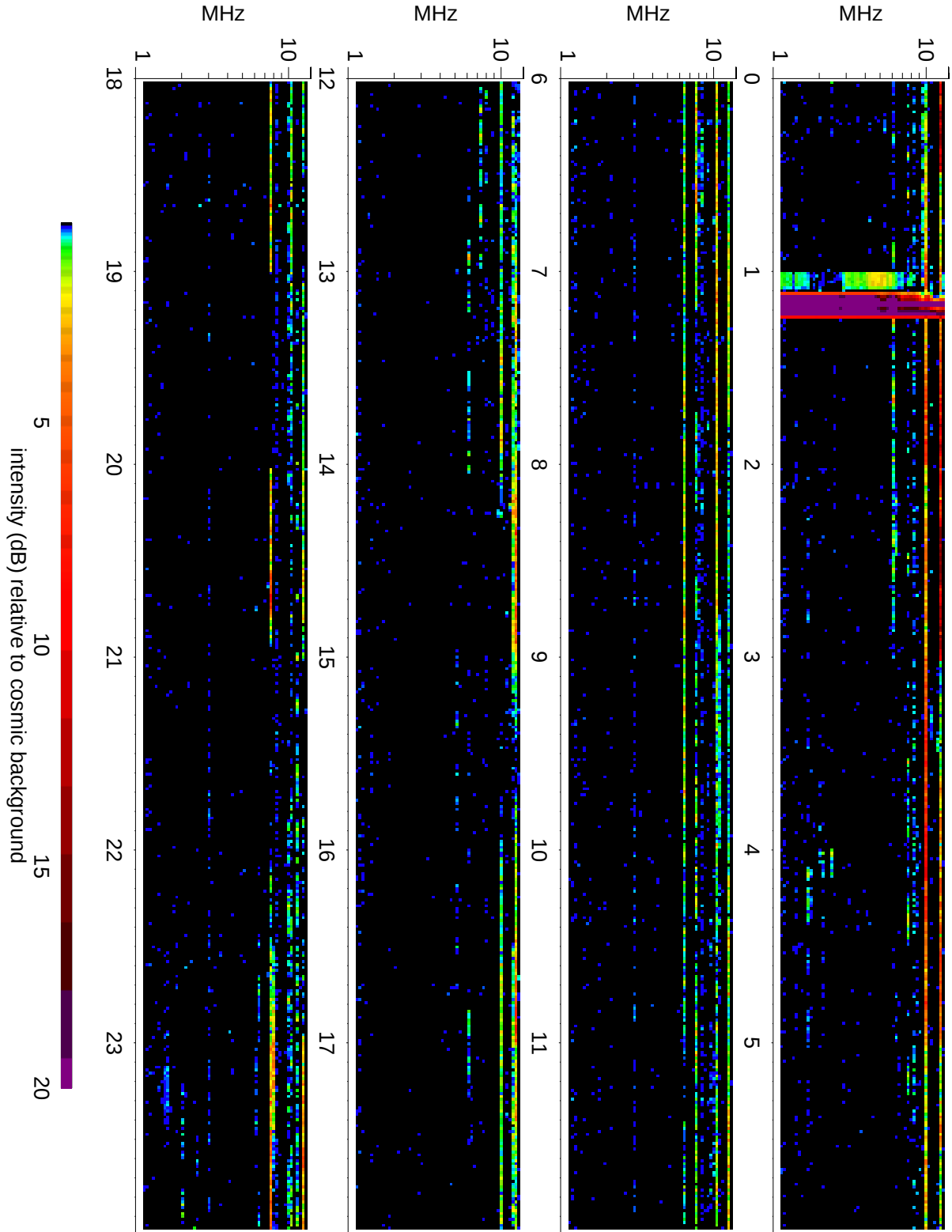
Wind Waves RAD2 receiver: 2007/08/10
