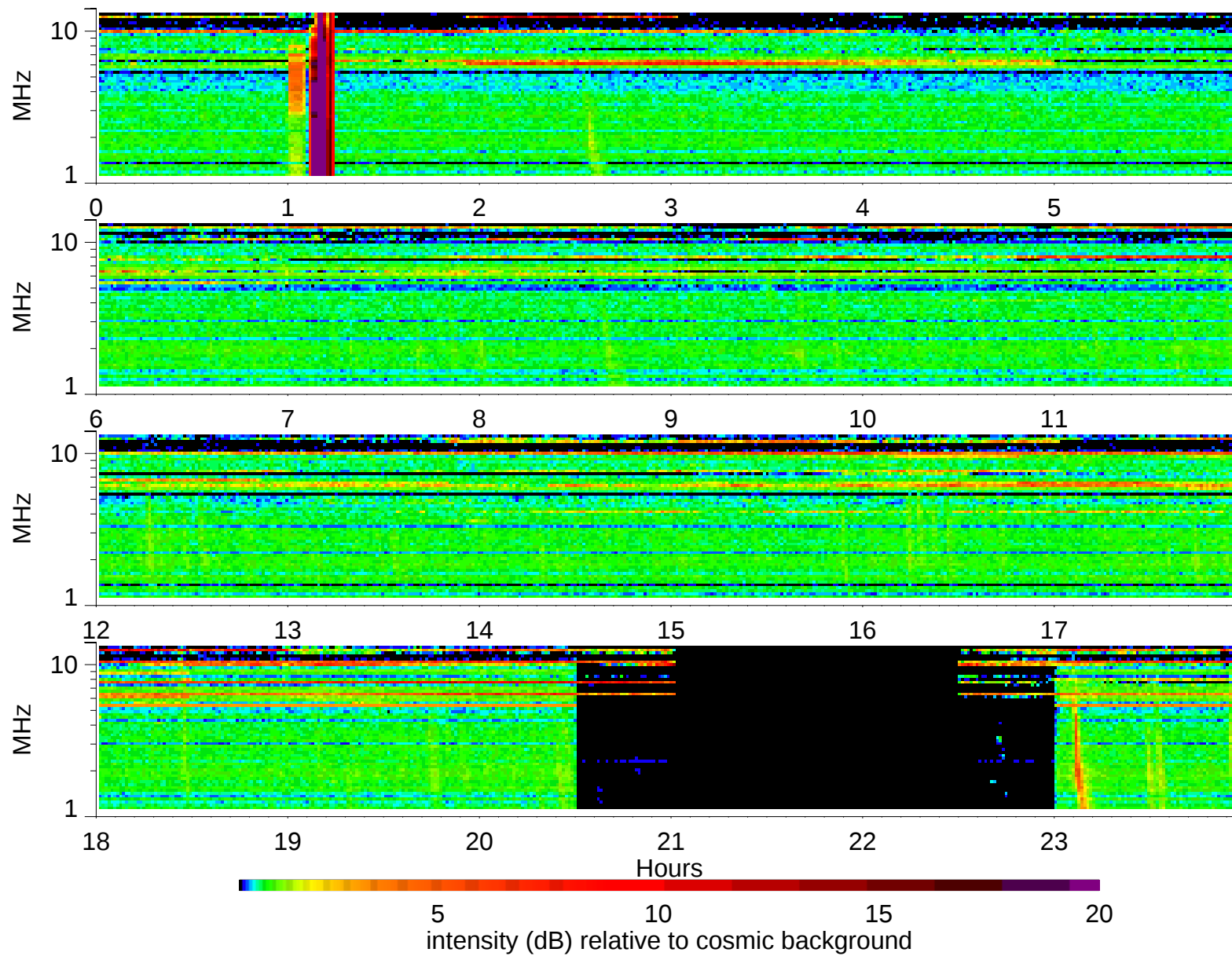
Wind Waves RAD2 receiver: 2003/11/30
