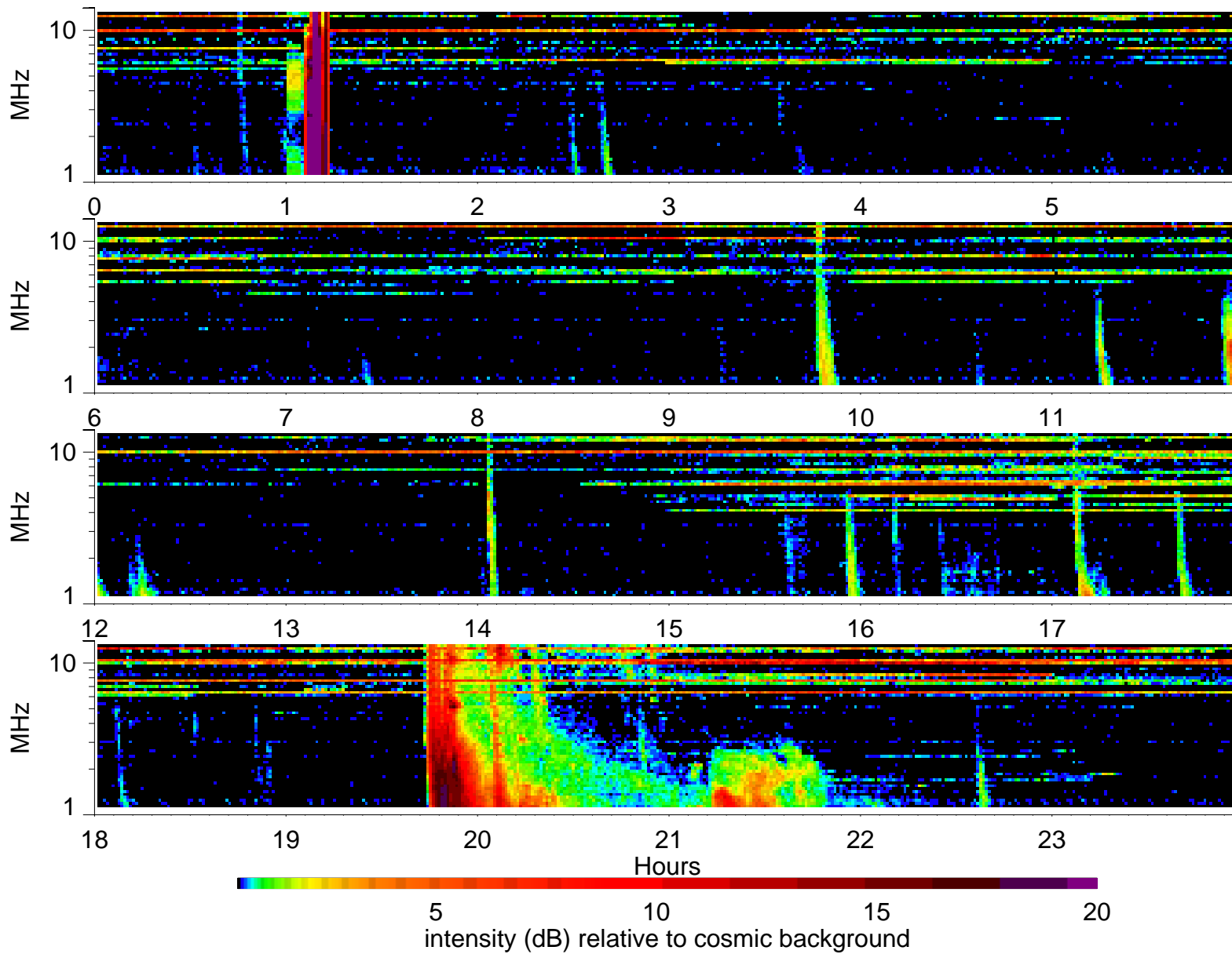
Wind Waves RAD2 receiver: 2003/11/4
