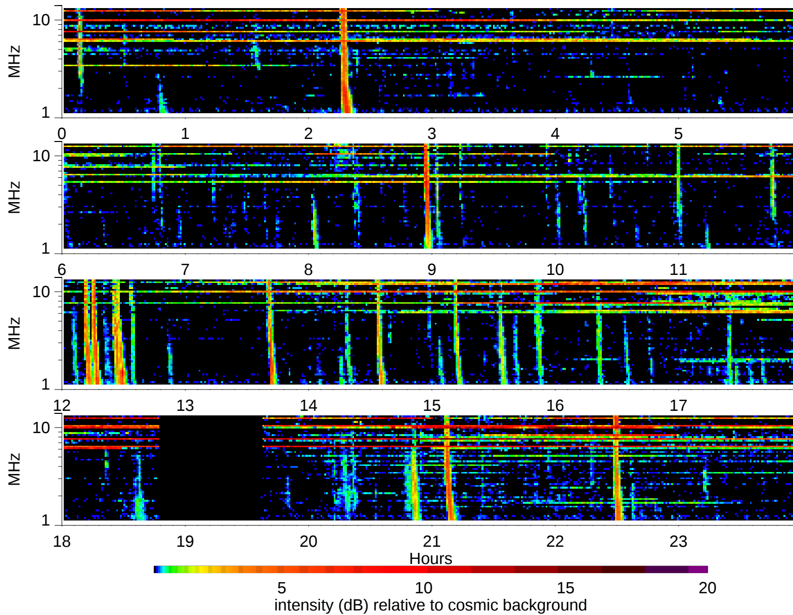
Wind Waves RAD2 receiver: 2003/10/30
