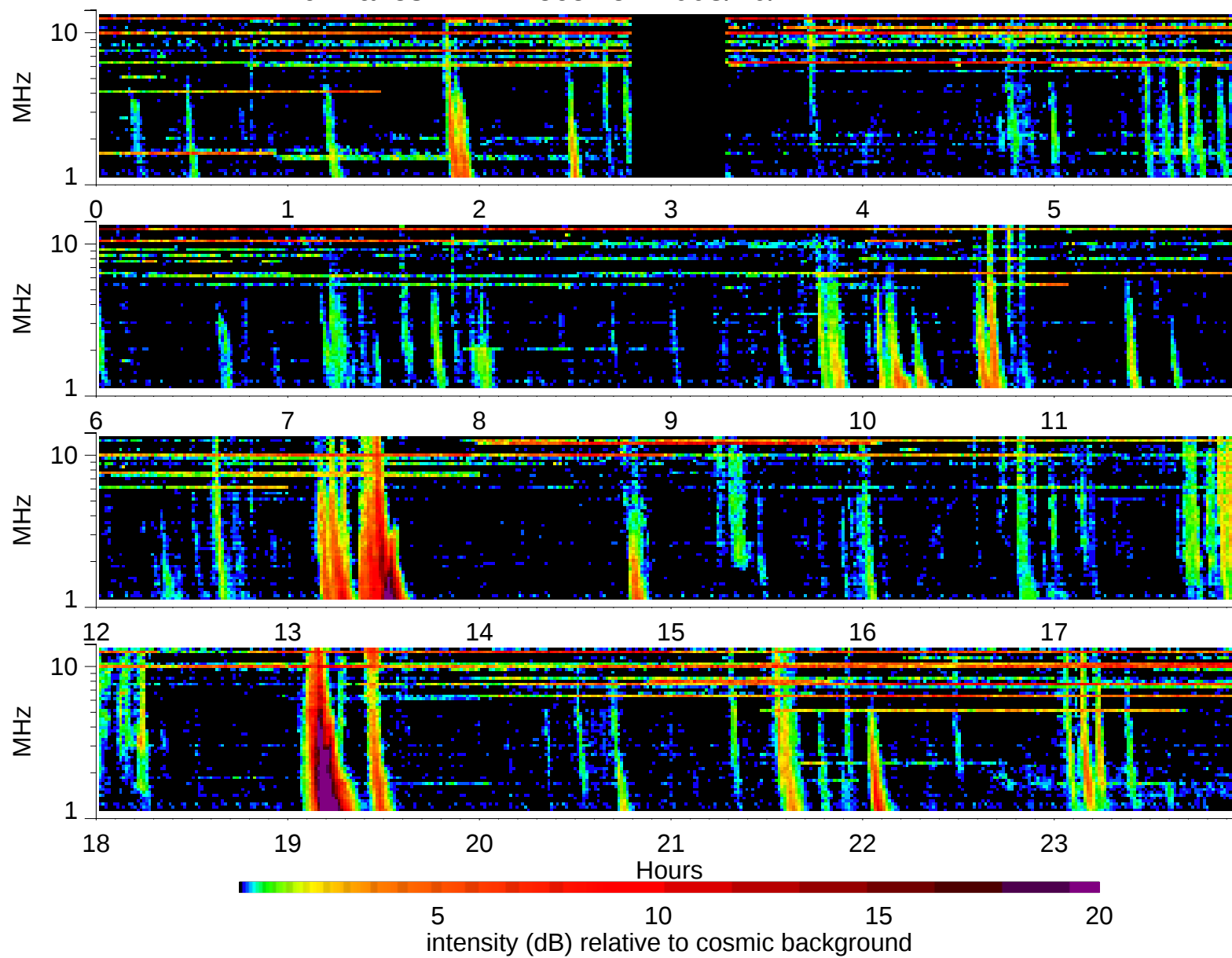
Wind Waves RAD2 receiver: 2003/10/4
