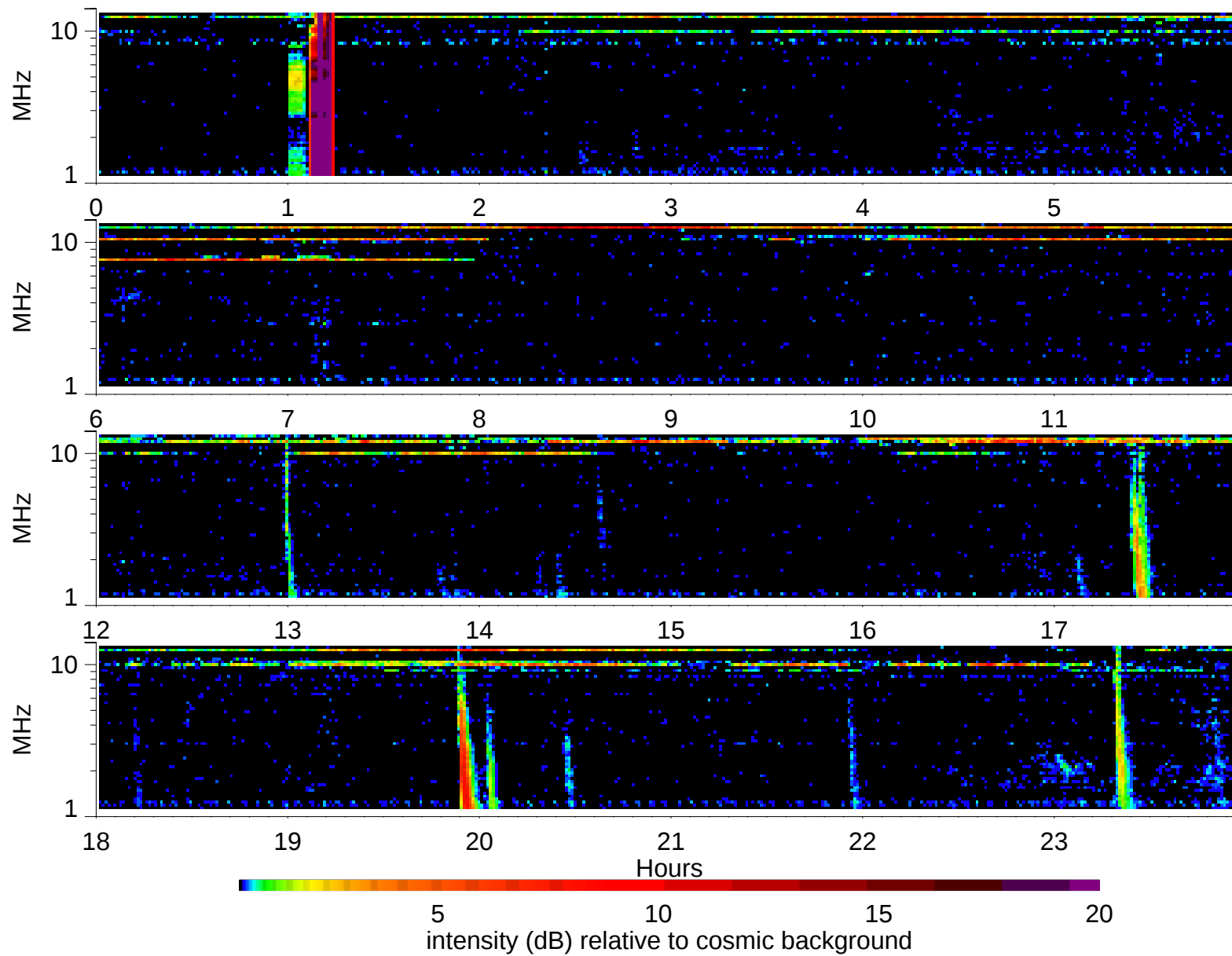
Wind Waves RAD2 receiver: 2003/7/31
