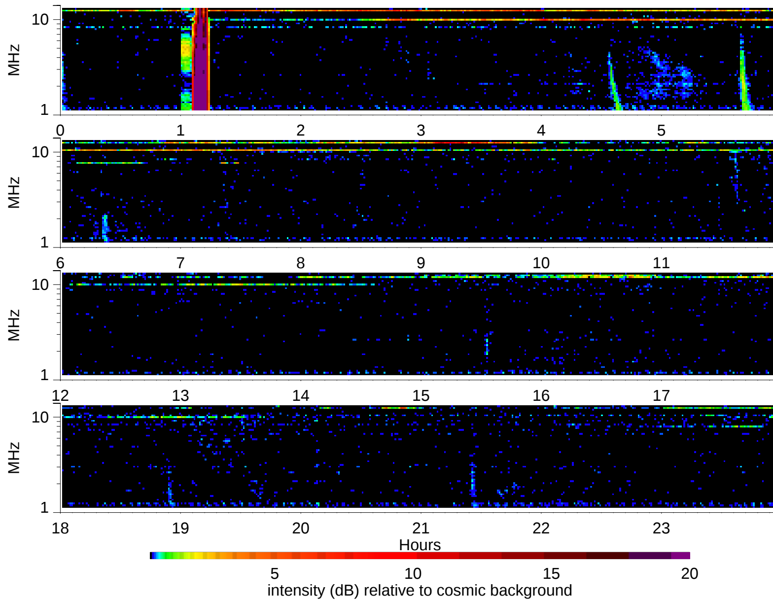
Wind Waves RAD2 receiver: 2003/6/25
