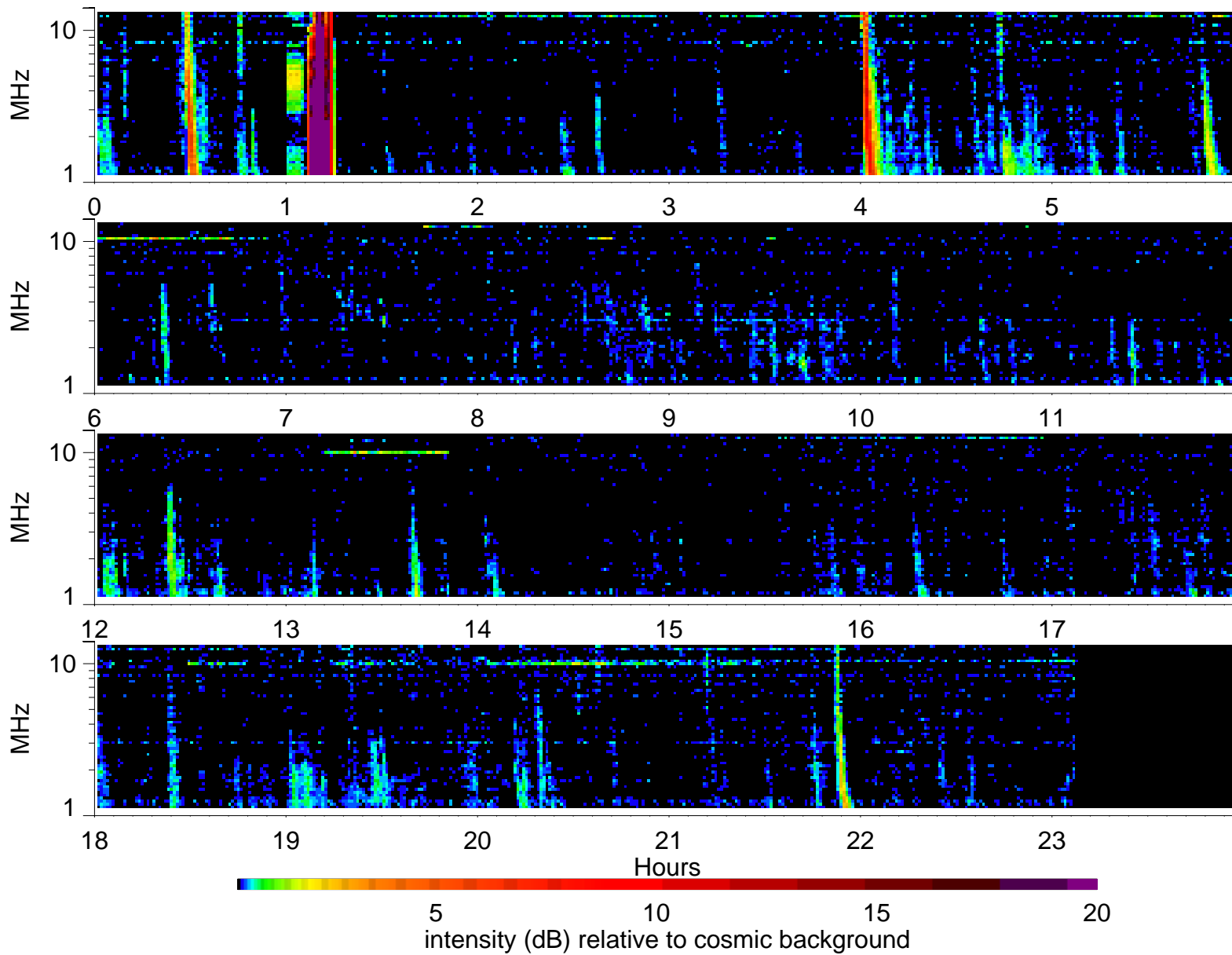
Wind Waves RAD2 receiver: 2003/4/28
