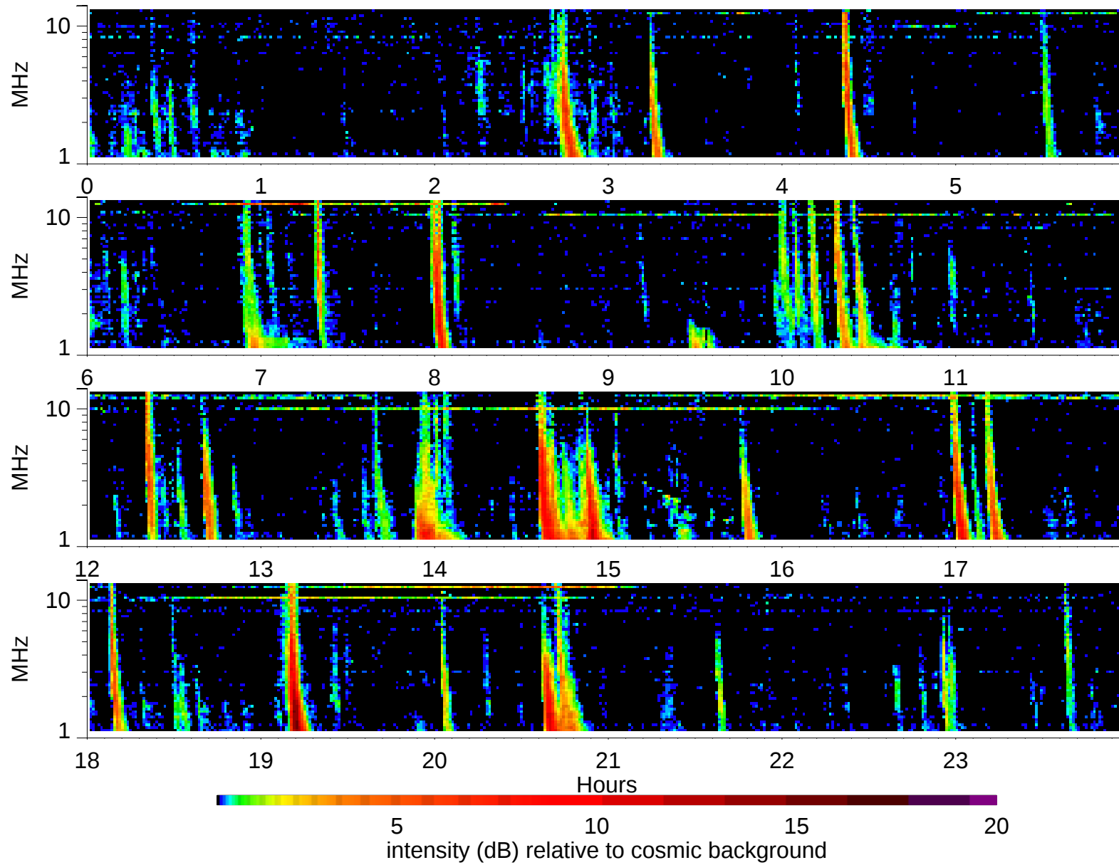
Wind Waves RAD2 receiver: 2003/4/1
