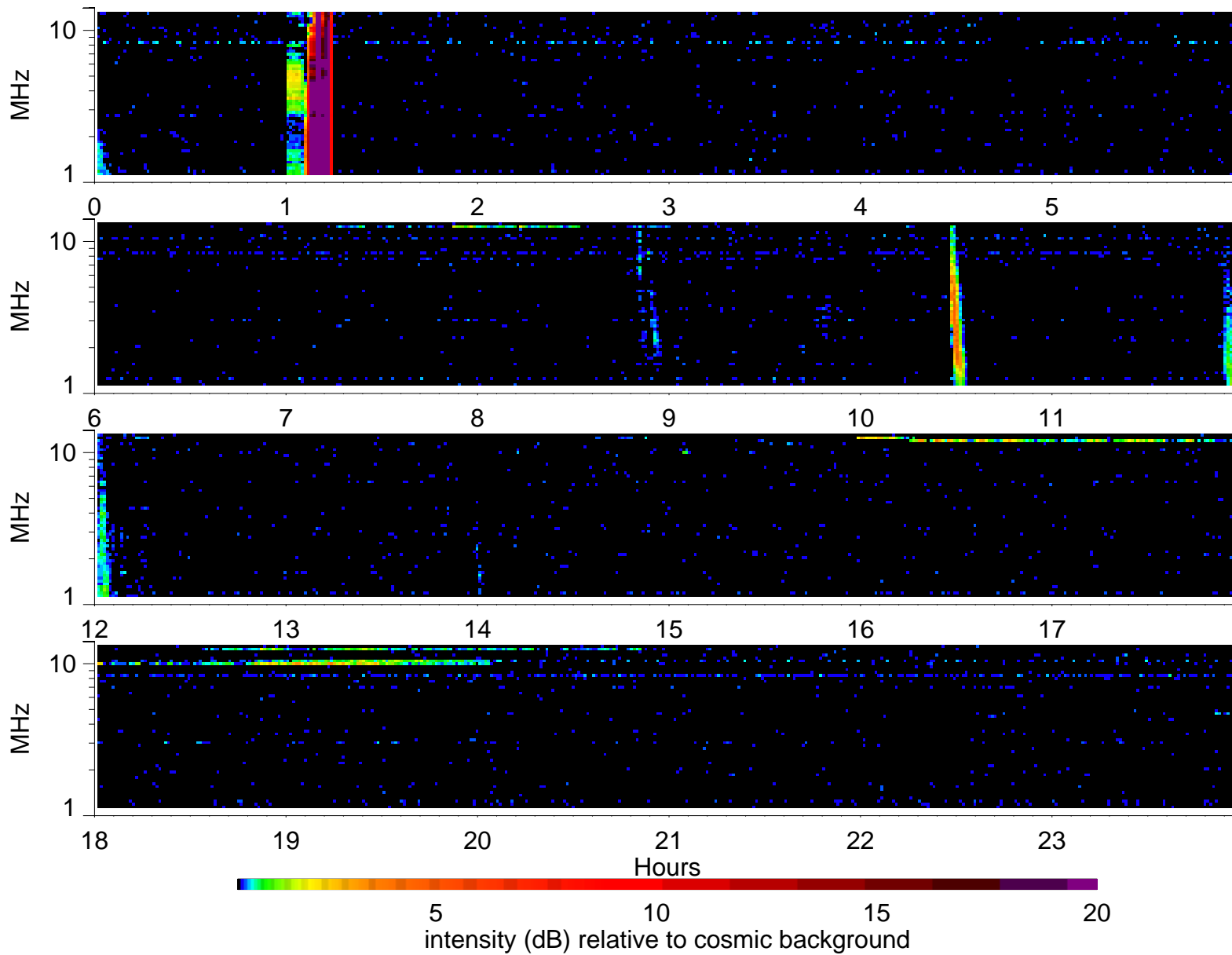
Wind Waves RAD2 receiver: 2003/3/23
