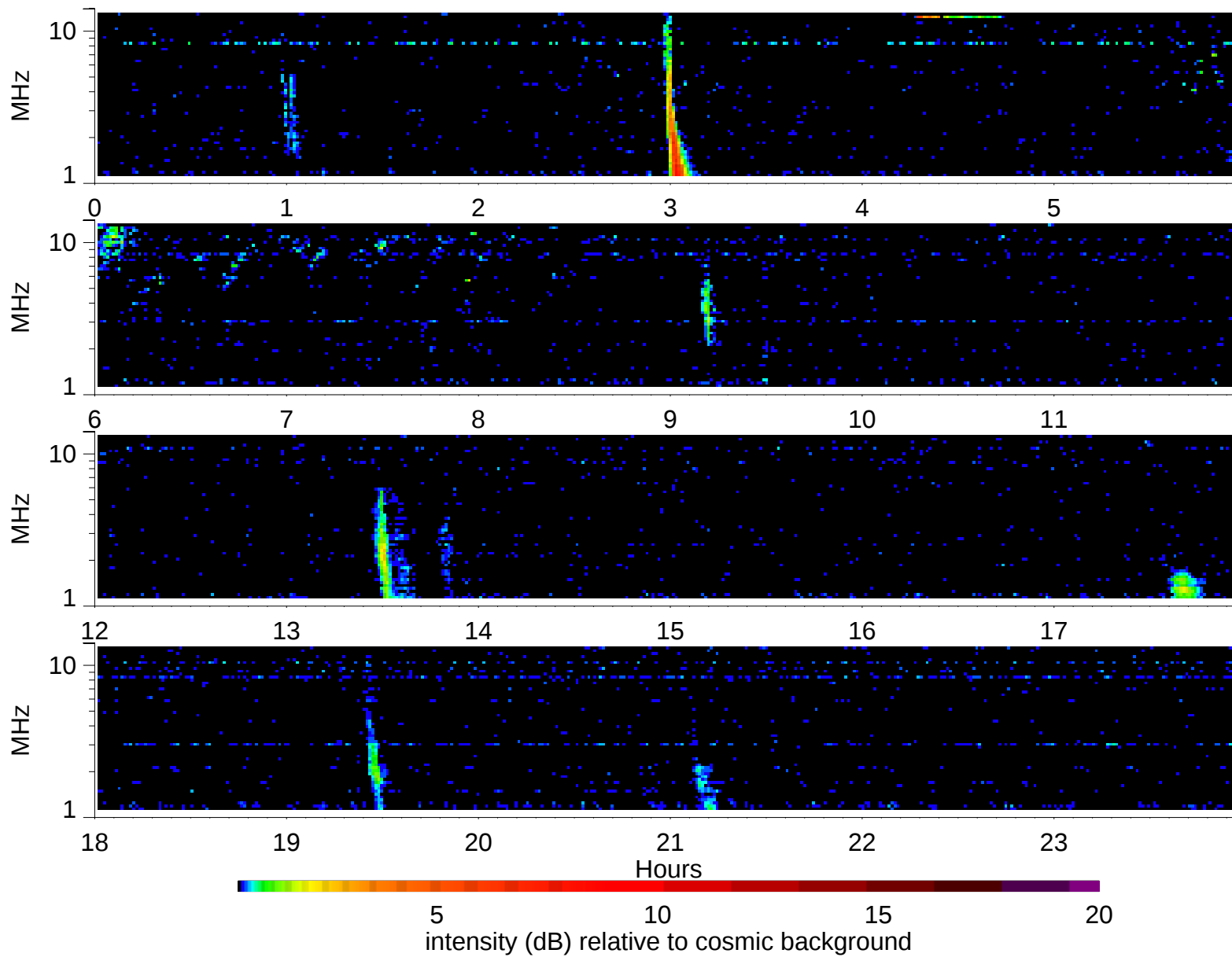
Wind Waves RAD2 receiver: 2003/2/26
