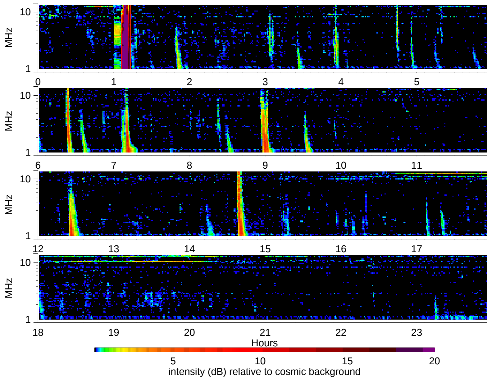
Wind Waves RAD2 receiver: 1999/9/1
