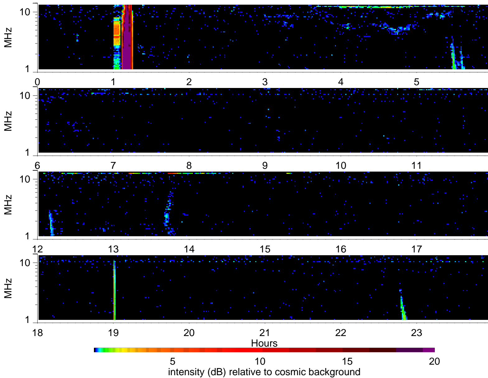
Wind Waves RAD2 receiver: 1997/12/28
