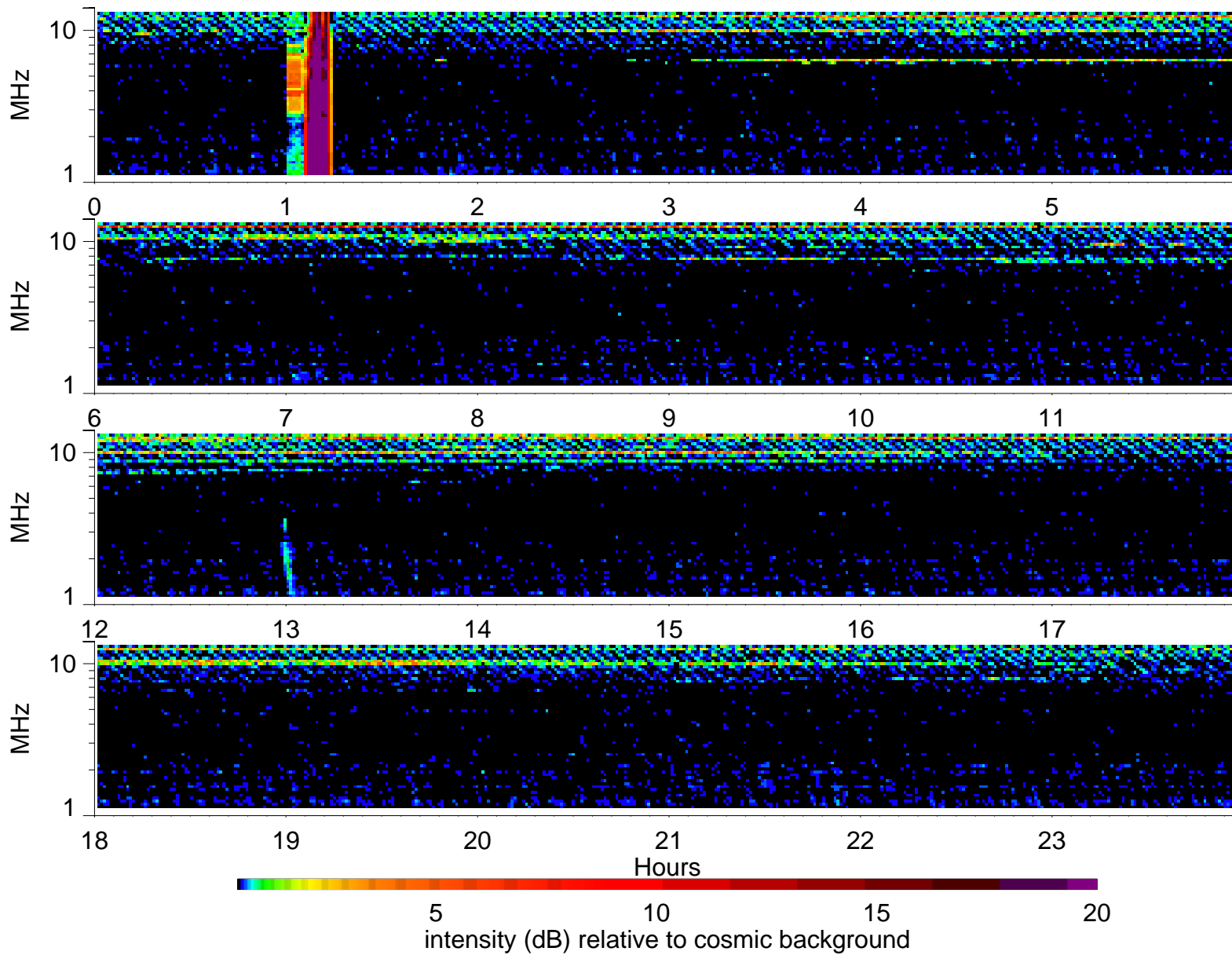
Wind Waves RAD2 receiver: 1996/7/30
